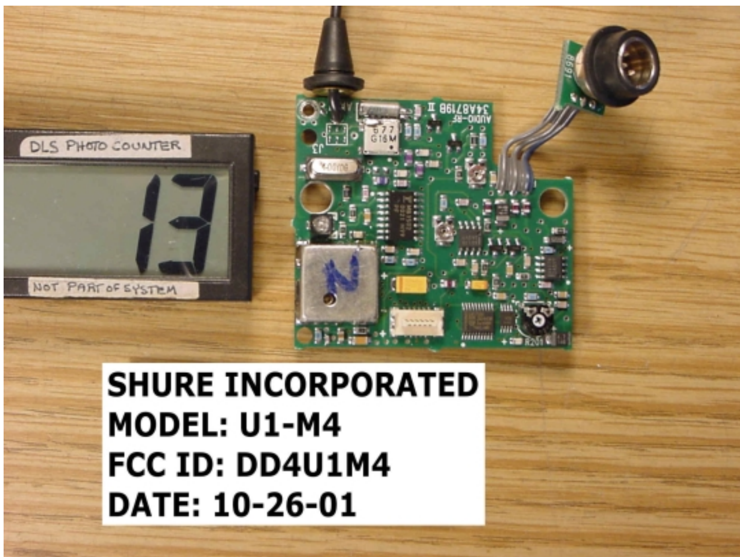
Audio – RF Board Side 1
