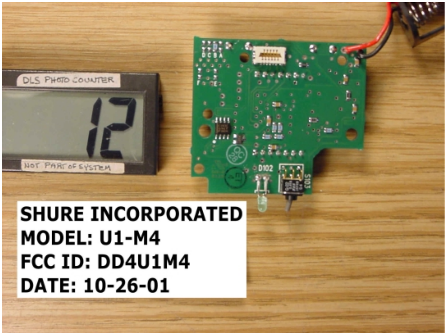
Display Board Side 2
