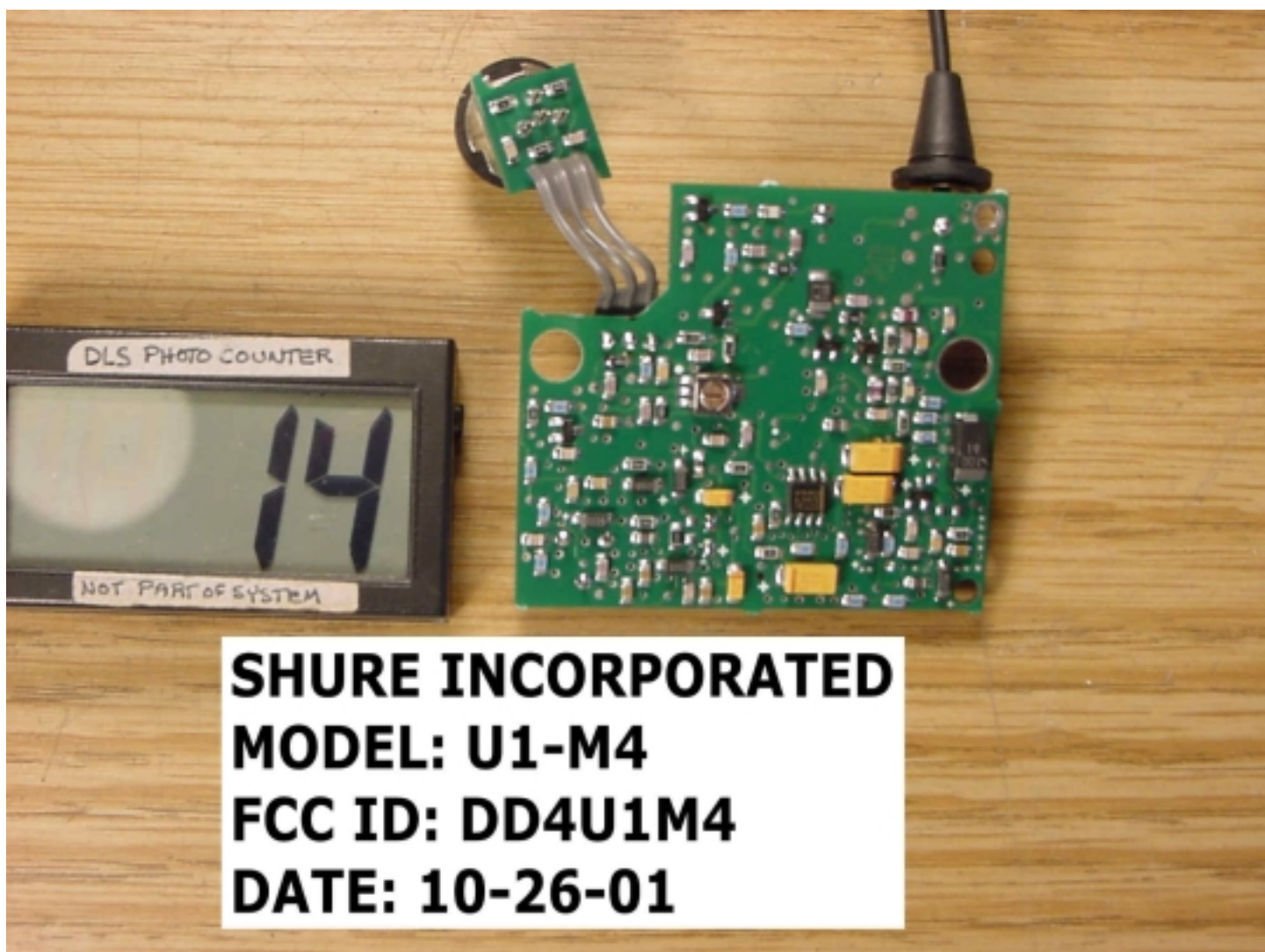
Audio – RF Board Side 2
