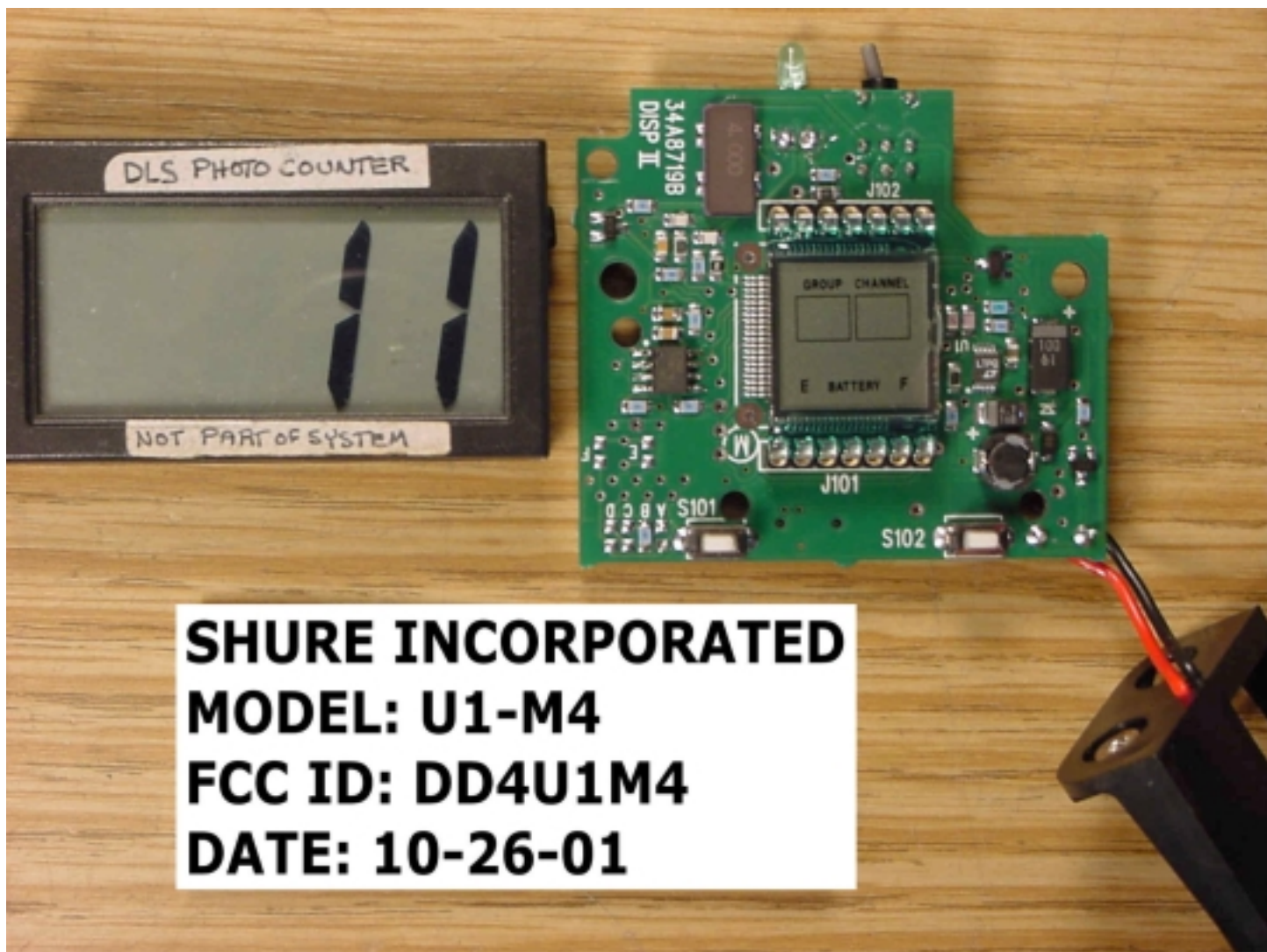
Display Board Side 1
