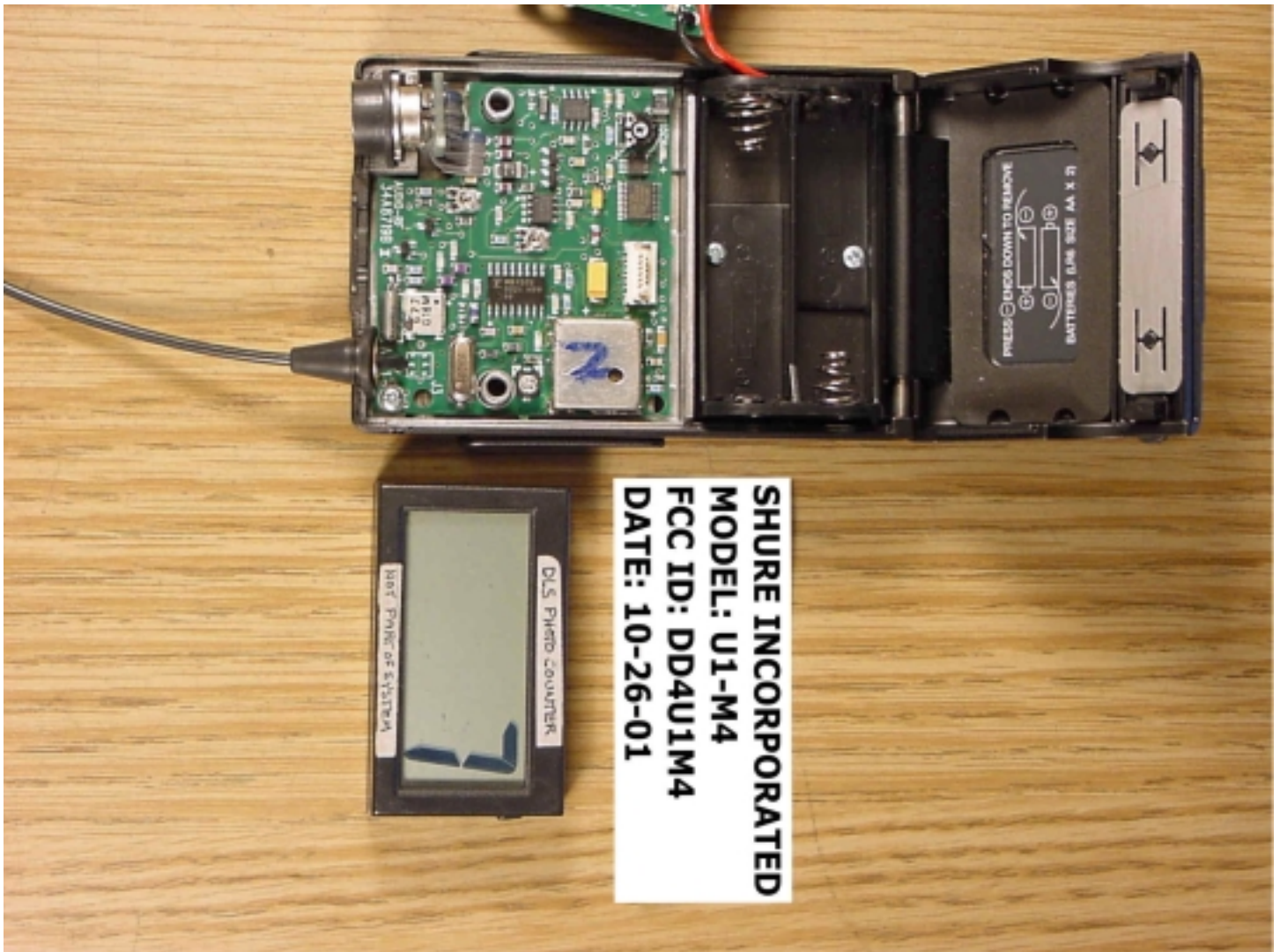
Display Board Removed
