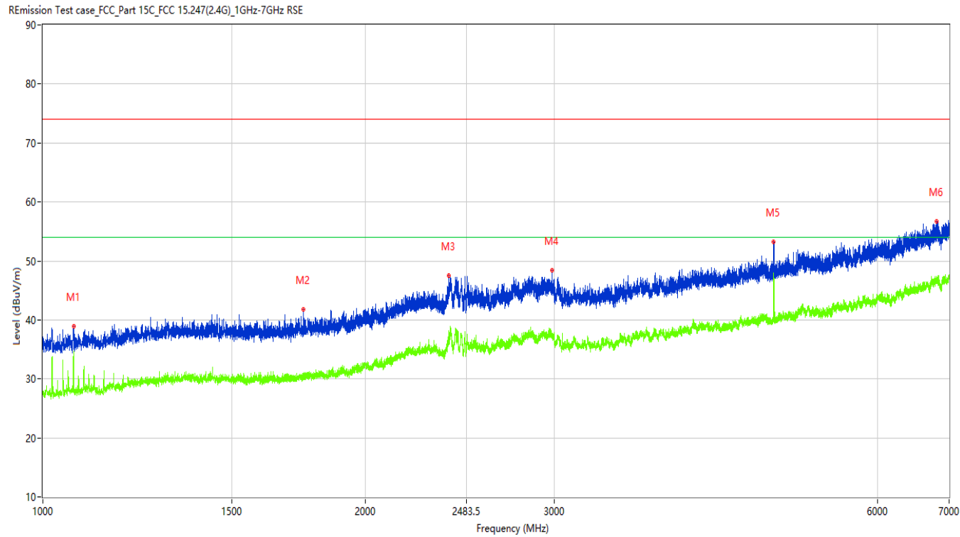
Figure 57: Radiated Emission, BLE-2M, 2402MHz_1GHz_7GHz Horizontal polarization
