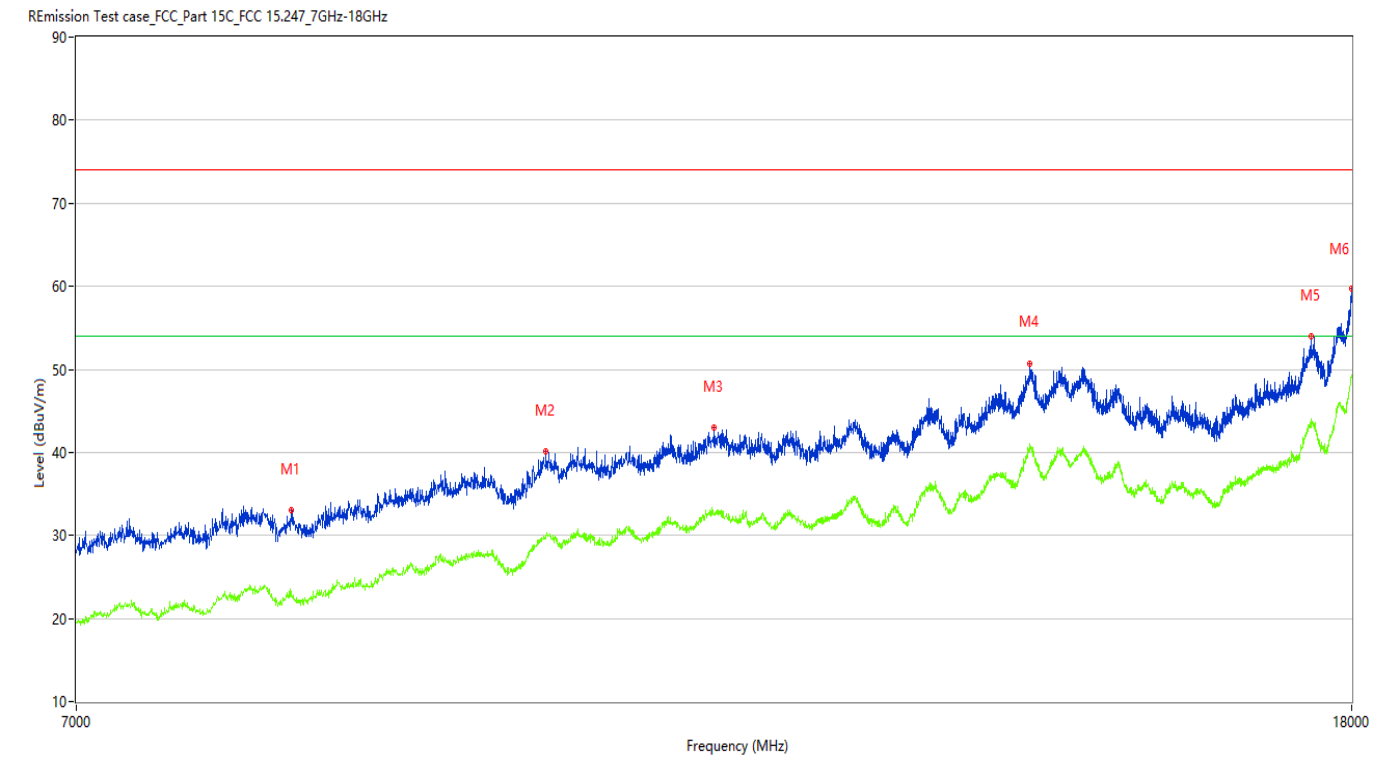
Figure 72: Radiated Emission, BLE-2M, 2402MHz_7GHz_18GHz Horizontal polarization
