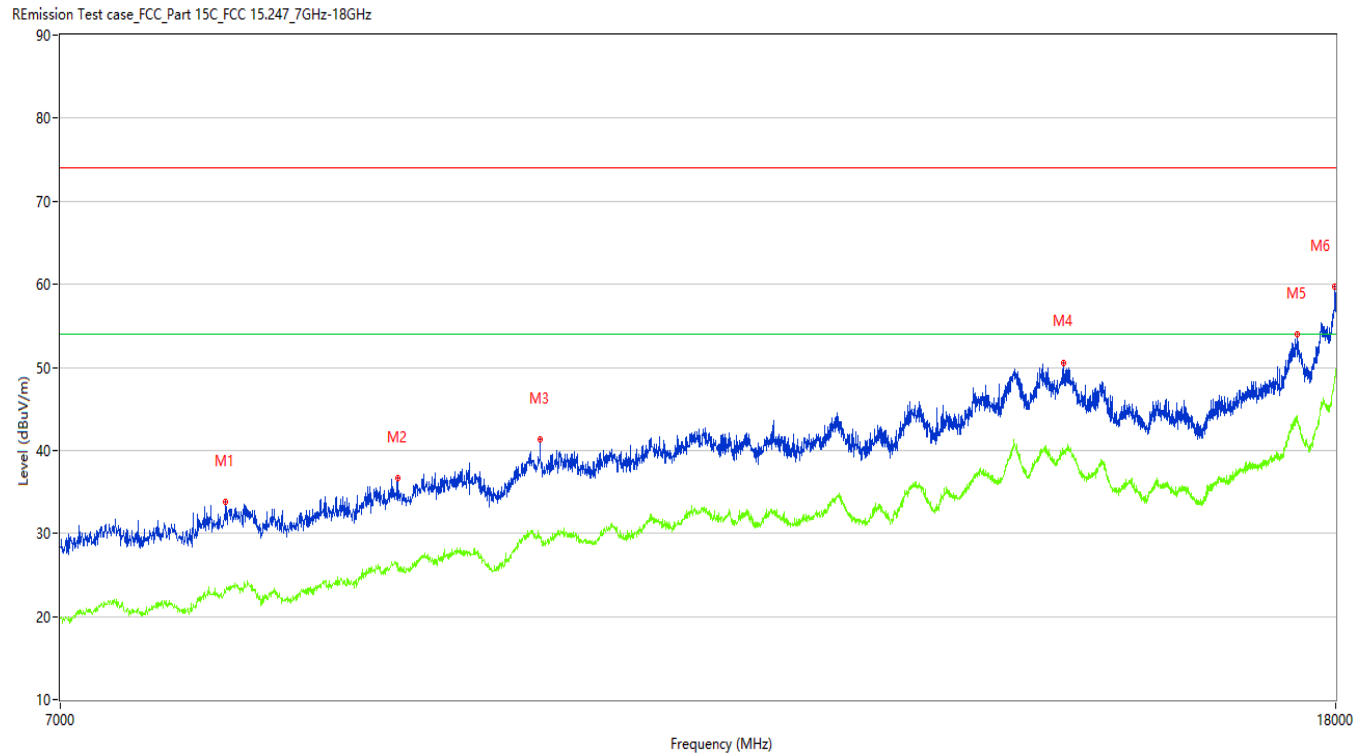
Figure 76: Radiated Emission, BLE-2M, 2480MHz_7GHz_18GHz Horizontal polarization
