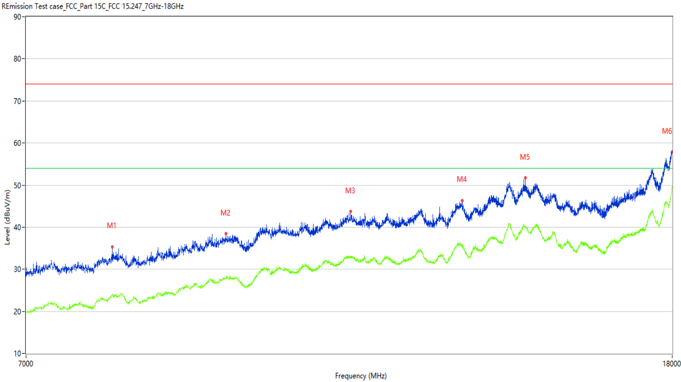
Figure 51: Radiated Emission, BLE-1M, 2402MHz_7GHz_18GHz Horizontal polarization
