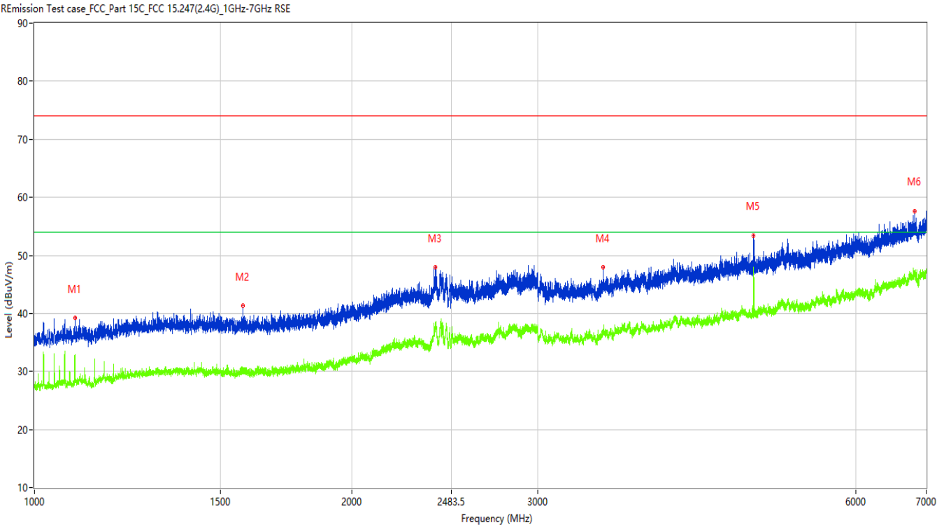
Figure 71: Radiated Emission, BLE-2M, 2402MHz_1GHz_7GHz Horizontal polarization
