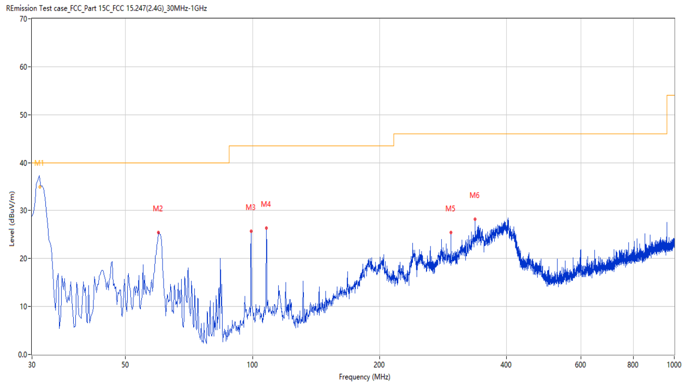
Figure 70: Radiated Emission, BLE-2M, 2402MHz_30MHz_1GHz Horizontal polarization
