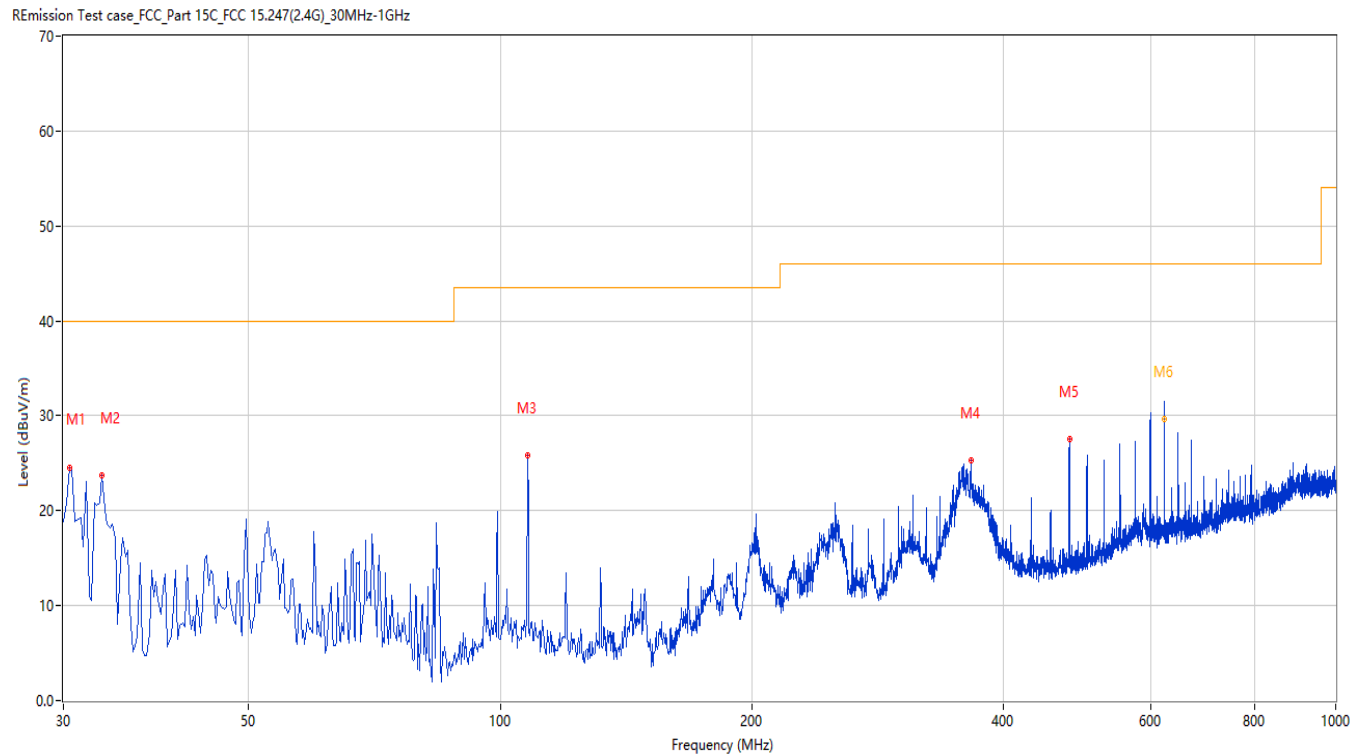
Figure 49: Radiated Emission, BLE-1M, 2402MHz_30MHz_1GHz Horizontal polarization
