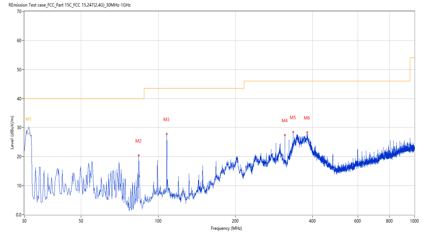
Figure 56: Radiated Emission, BLE-2M, 2402MHz_30MHz_1GHz Horizontal polarization
