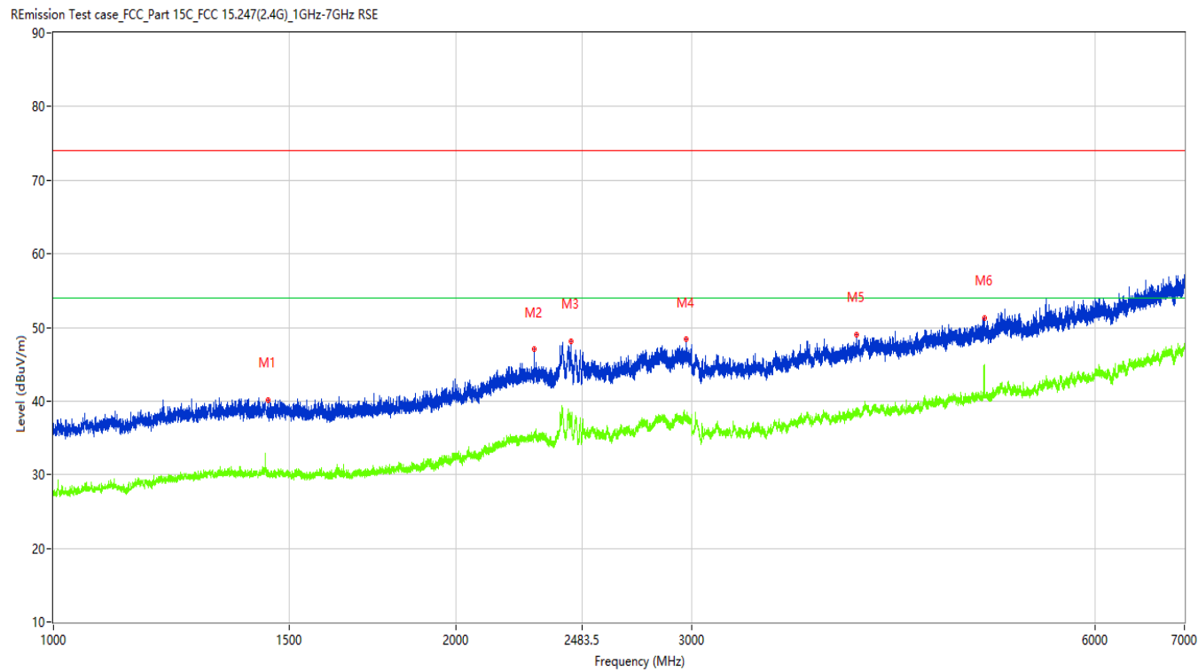
Figure 54: Radiated Emission, BLE-1M, 2480MHz_1GHz_7GHz Horizontal polarization
