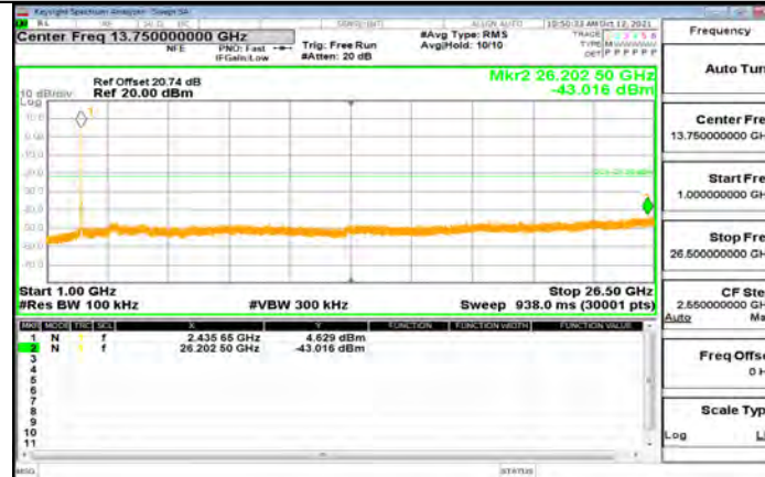
11G_Ant2_2437_1000~26500
