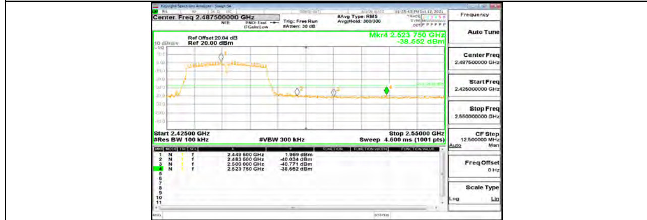
11N40MIMO_Ant1_High_2452
