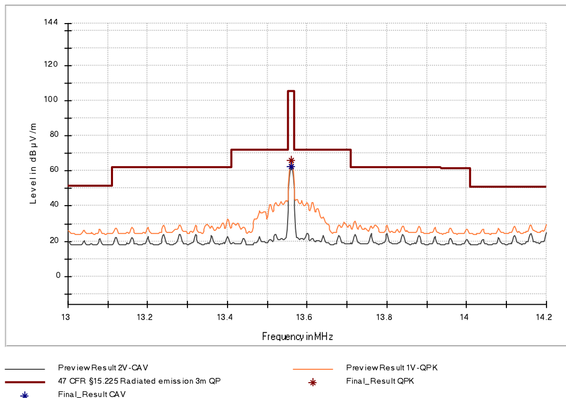
Figure 8: Chart of emission within the band 13.110 MHz to 14.010 MHz, EUT in position Z, without tag, antenna in line at 3 m distance
