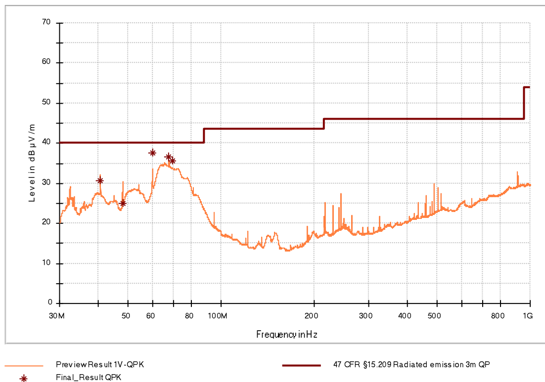
Figure 10: Chart of emissions test from 30 MHz to 1 GHz, EUT position Z, without tag, antenna vertical, at 3 m
