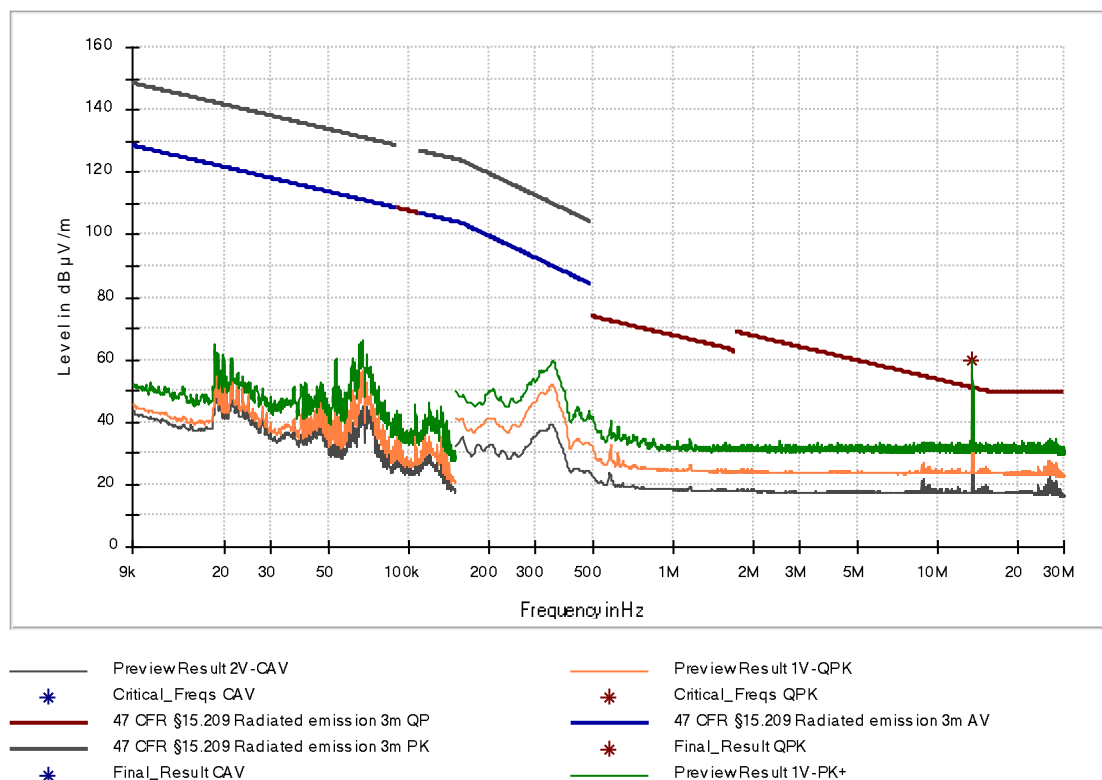
Figure 9: Chart of emissions test below 30 MHz, EUT position Z, without tag, antenna parallel at 3 m
