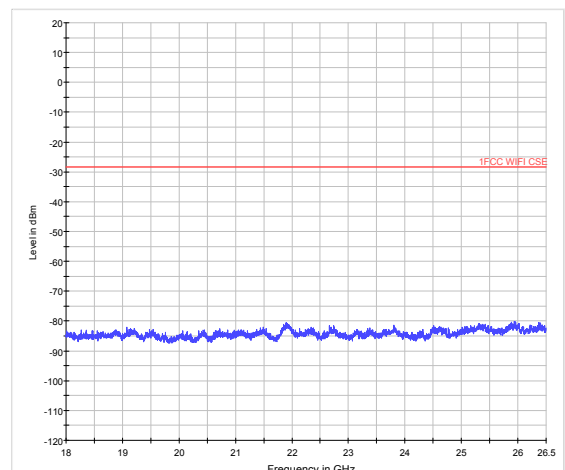
802.11n (HT40) CH9 18GHz to 26.5GHz
