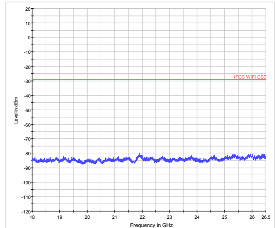
802.11n (HT40) CH6 18GHz to 26.5GHz
