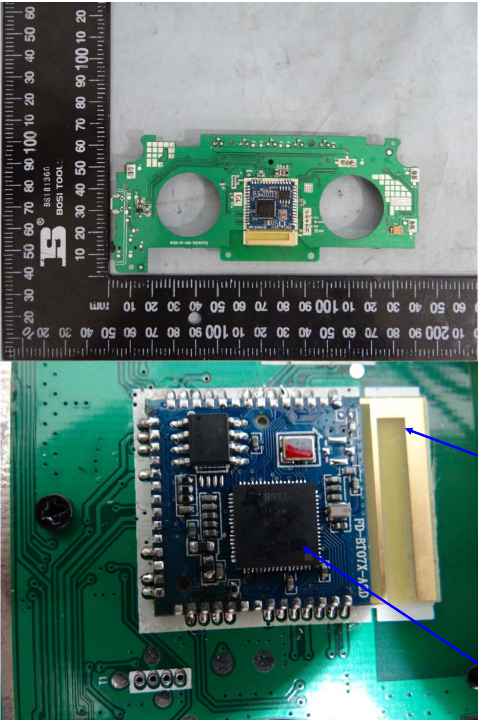
BT Antenna
