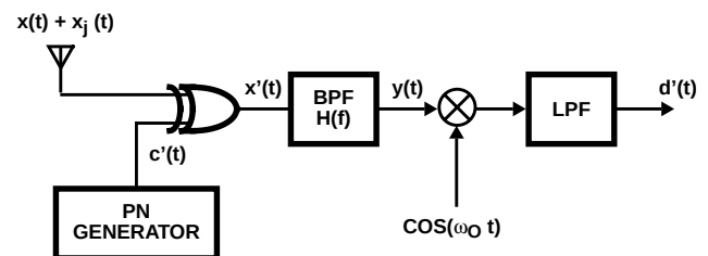
FIGURE 17. DSSS RECEIVER
