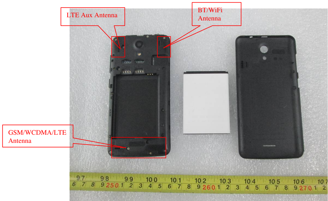
EUT – Cover off View 1
