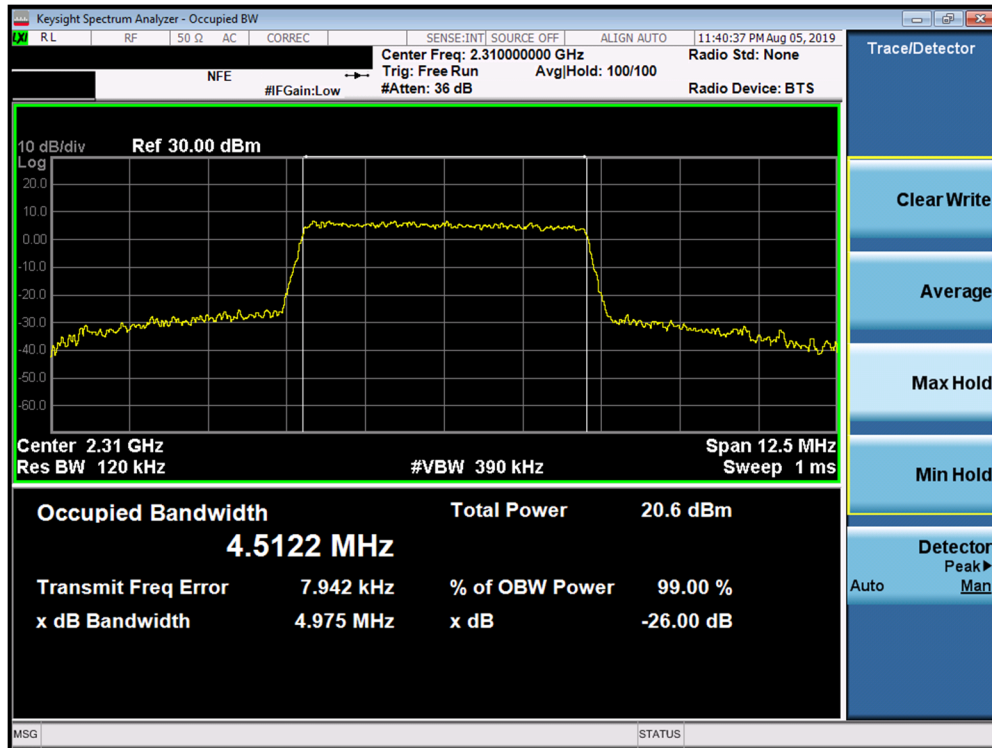
Plot 7-9. Occupied Bandwidth Plot (Band 30 - 5.0MHz 64-QAM - Full RB Configuration)
