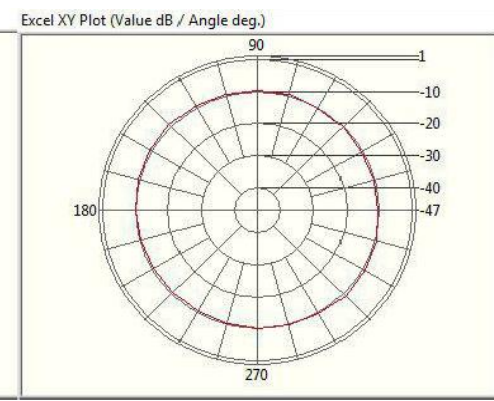
2.485GHz@Theta 0.0 Total
