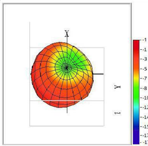
2.45GHzDown View
