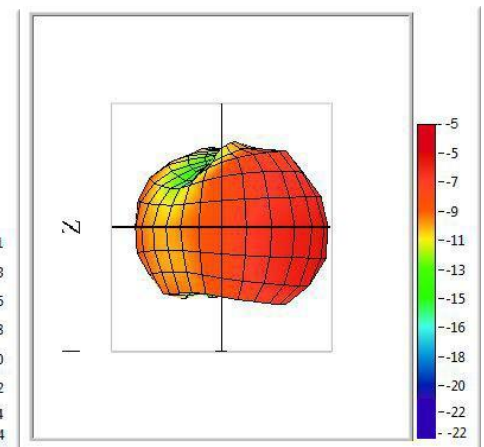
2.485GHzFront View
