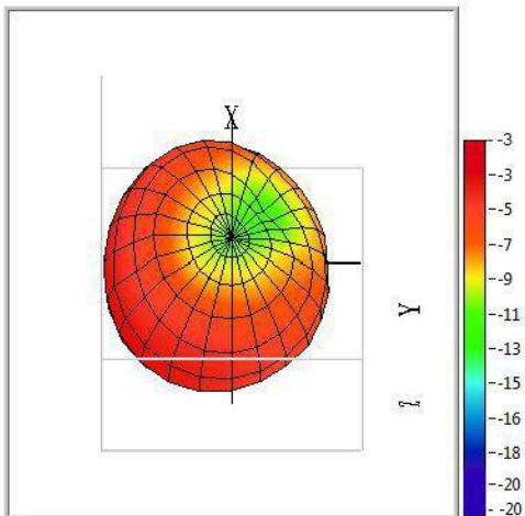
2.485GHzDown View
