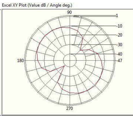
2.485GHz@Theta 0.0 Vertical
