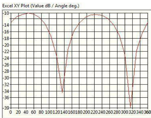
2.485GHz@Theta 0.0 Horizontal
