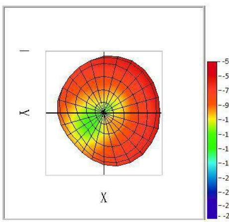
2.485GHzUp View
