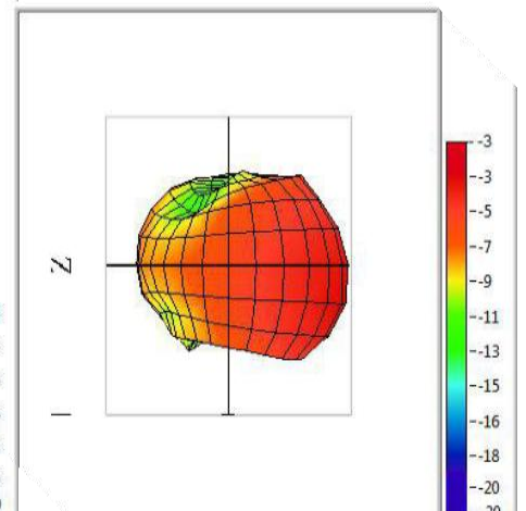
2.485GHzFront View
