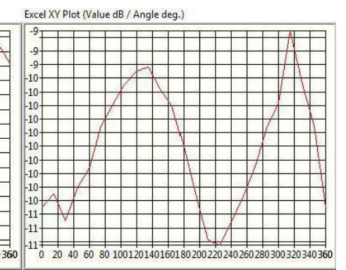
2.485GHz@Theta 0.0 Total
