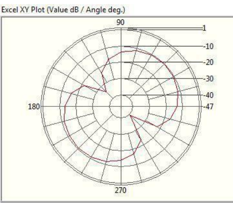
2.485GHz@Theta 0.0 Horizontal
