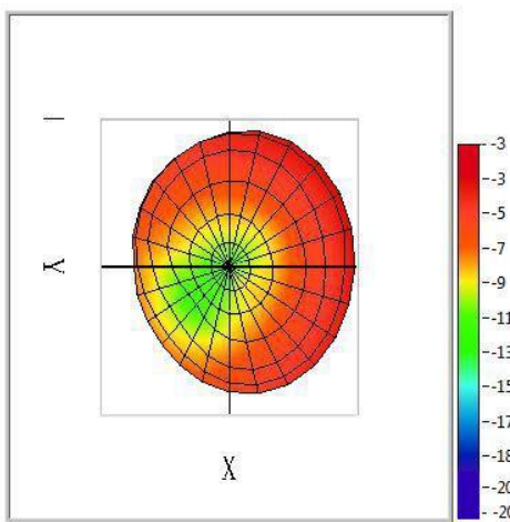
2.485GHzUp View
