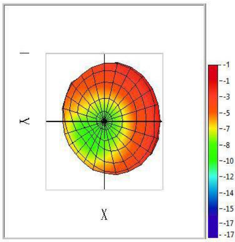
2.45GHzUp View
