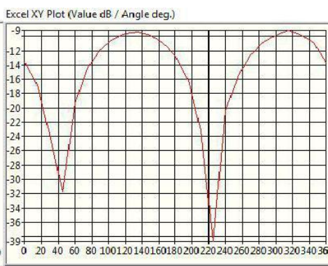
2.485GHz@Theta 0.0 Vertical
