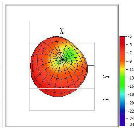
2.485GHzDown View
