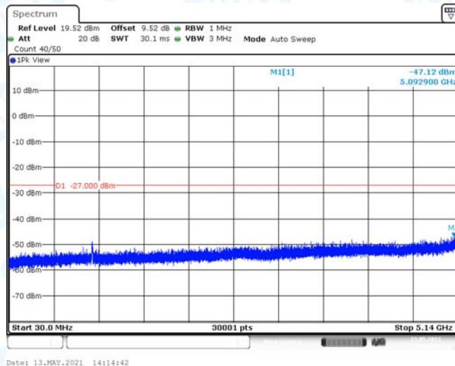
11A-MIMO_Ant4_5180_30~5140
