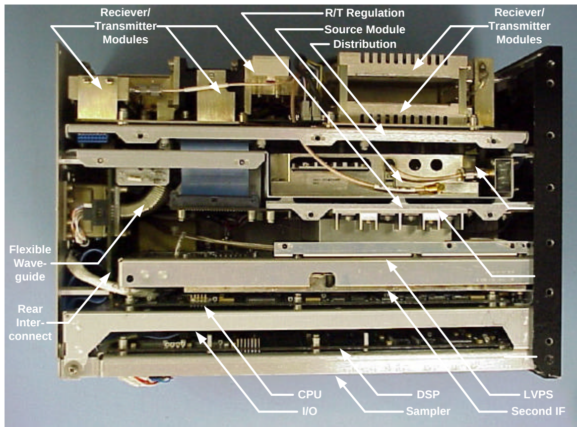
Figure I-1. Top Plate Removed
