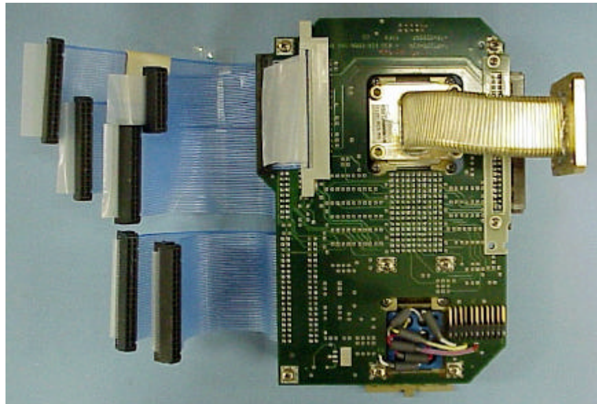
Figure I-21 Rear Interconnect Front
