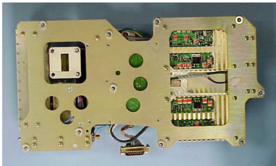
Figure I-14. Receiver / Transmitter Rear
