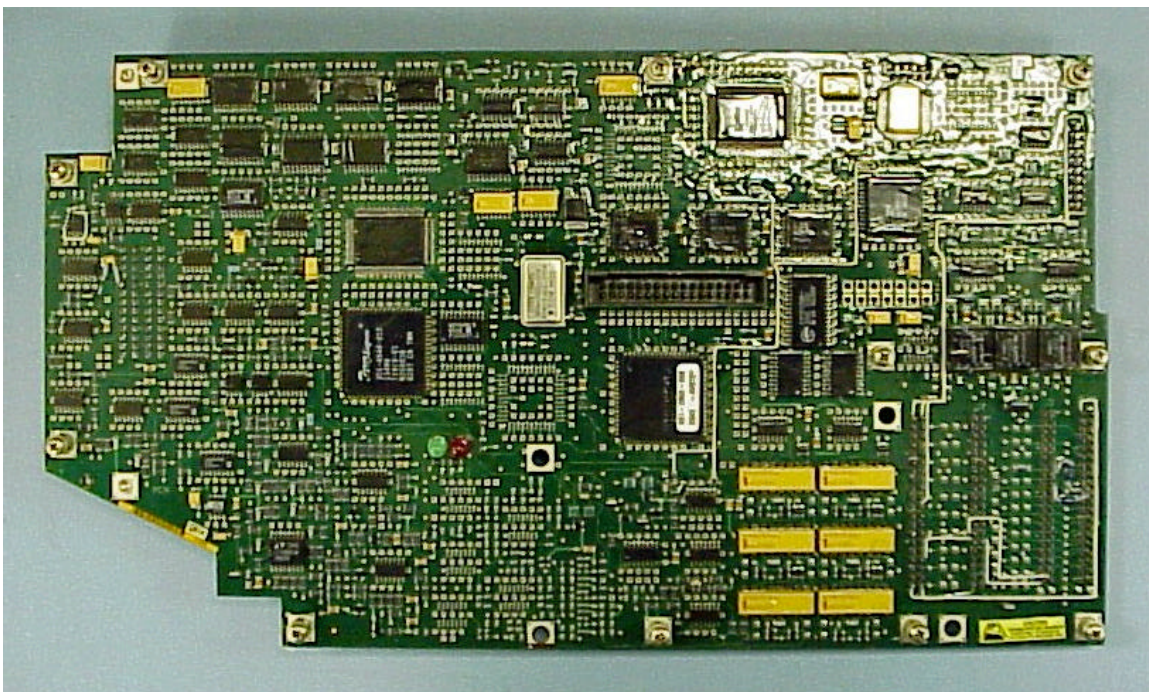
Figure I-19. CPU Front
