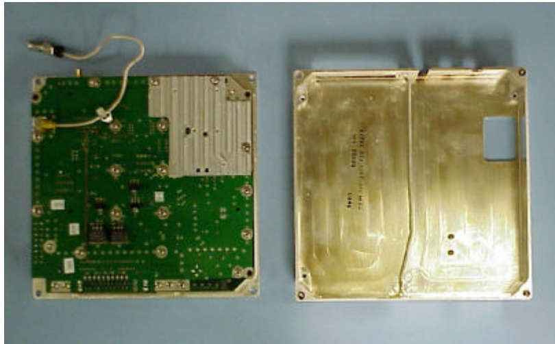
Figure I-6. Source Opened, Top Cover Removed
