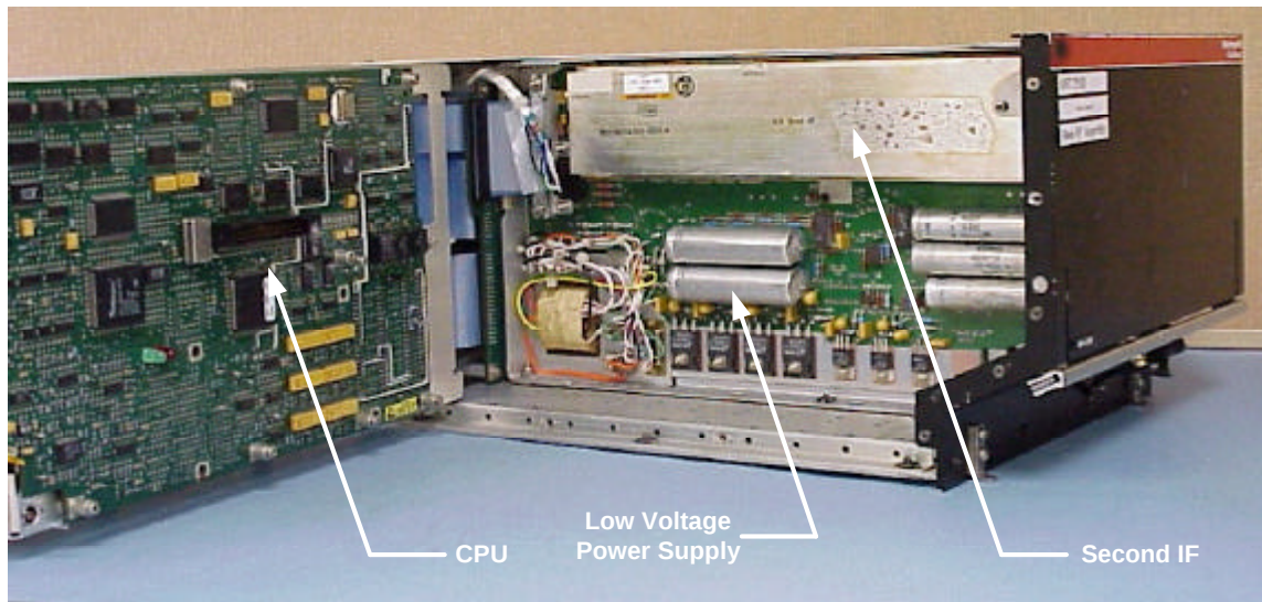
Figure I-2. Chassis Left Open
