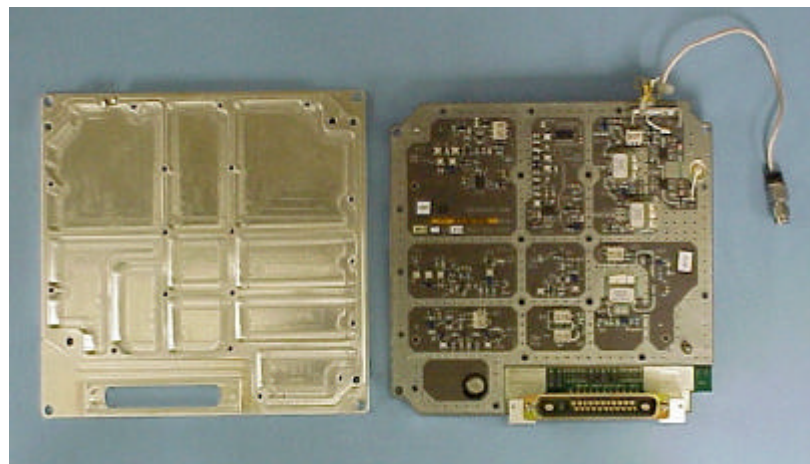
Figure I-7. Source Opened, Rear Cover Removed
