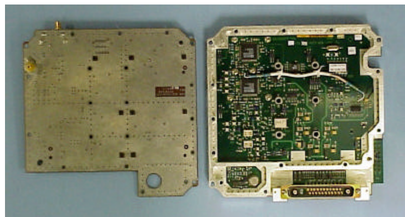
Figure I-8. Source, RF Rear, Digital Top
