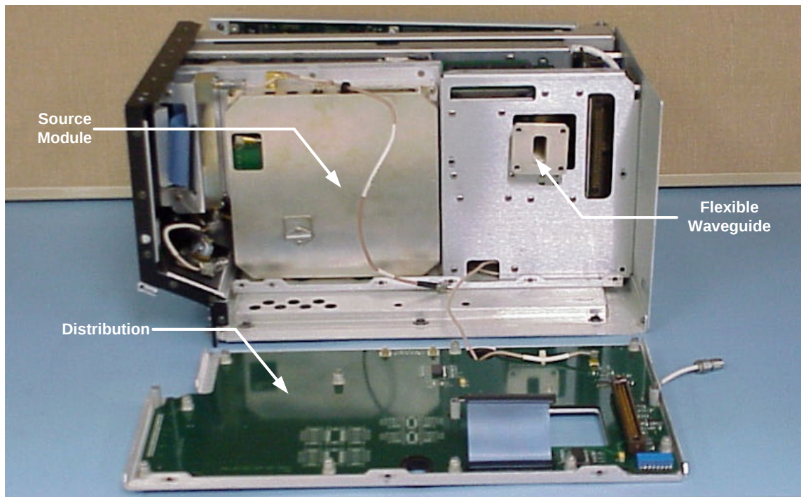
Figure I-4. Chassis Right Open
