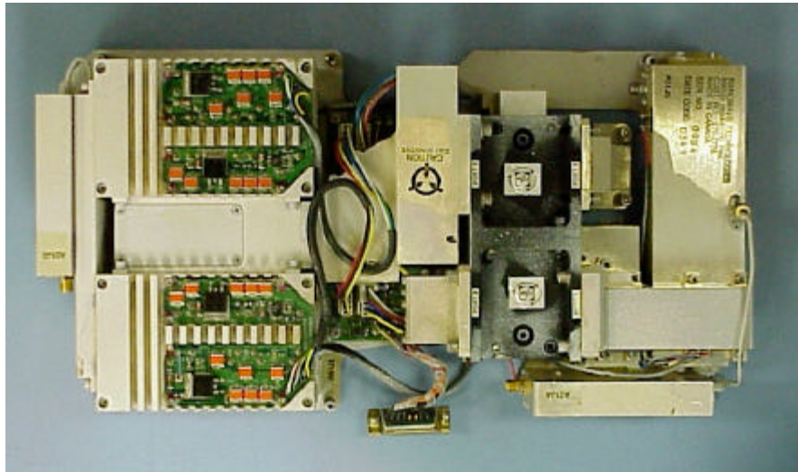
Figure I-13. Receiver / Transmitter Right
