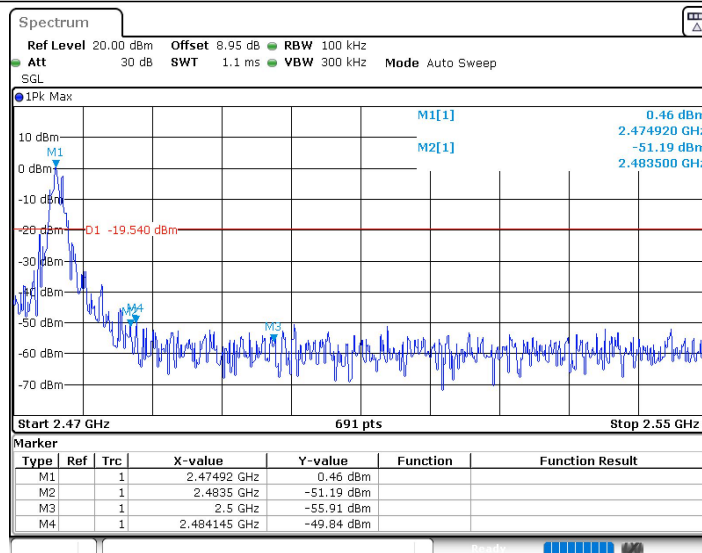
ZIGB_Ant1_High_2475
