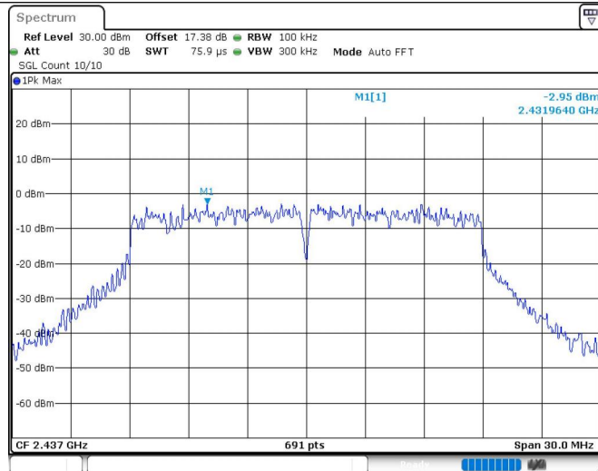
11N20SISO_Ant1_2437_0~Reference
