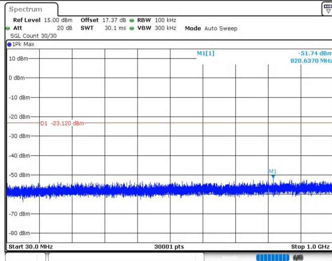
11N20SISO_Ant1_2462_30~1000
