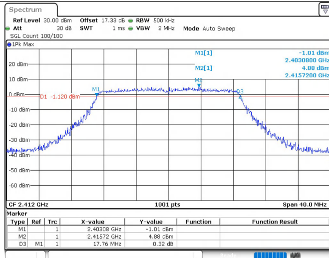
11N20SISO_Ant1_2412
