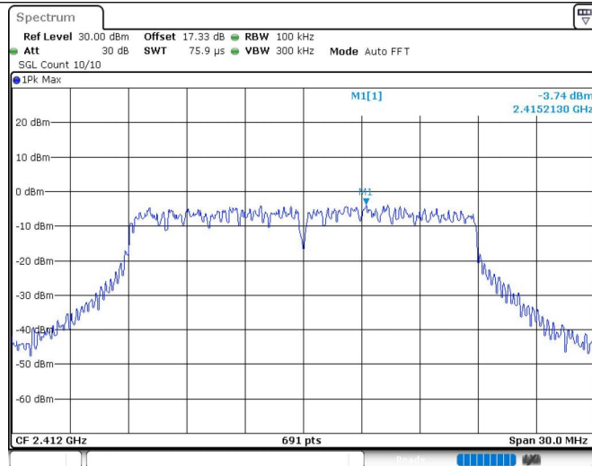
11N20SISO_Ant1_2412_0~Reference
