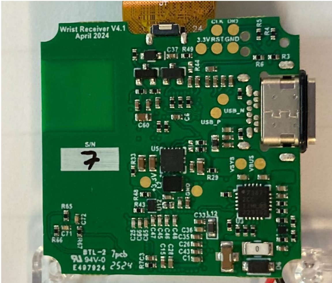
Figure 6. PCB Board Top View
