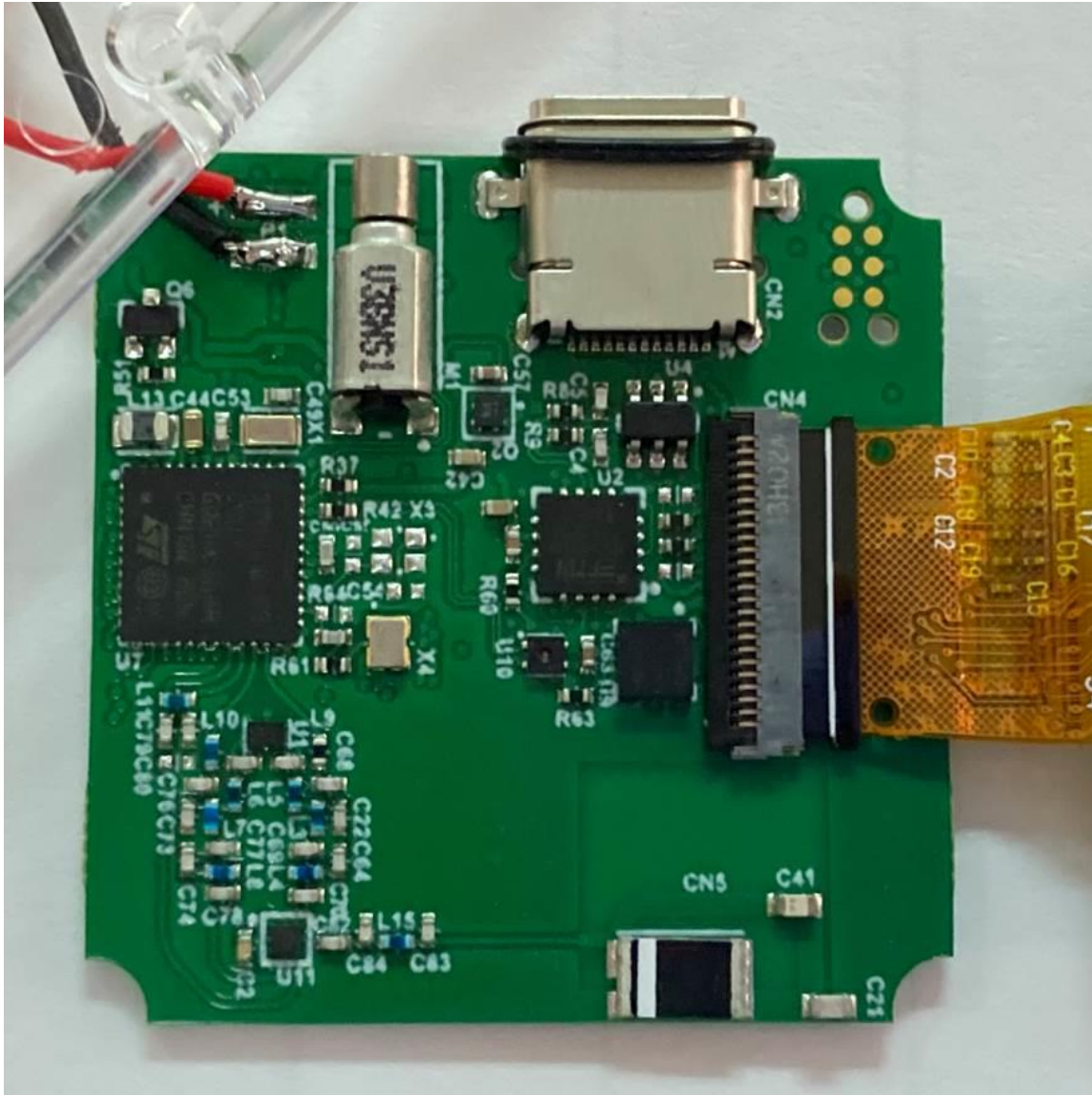
Figure 7. PCB Bottom View
