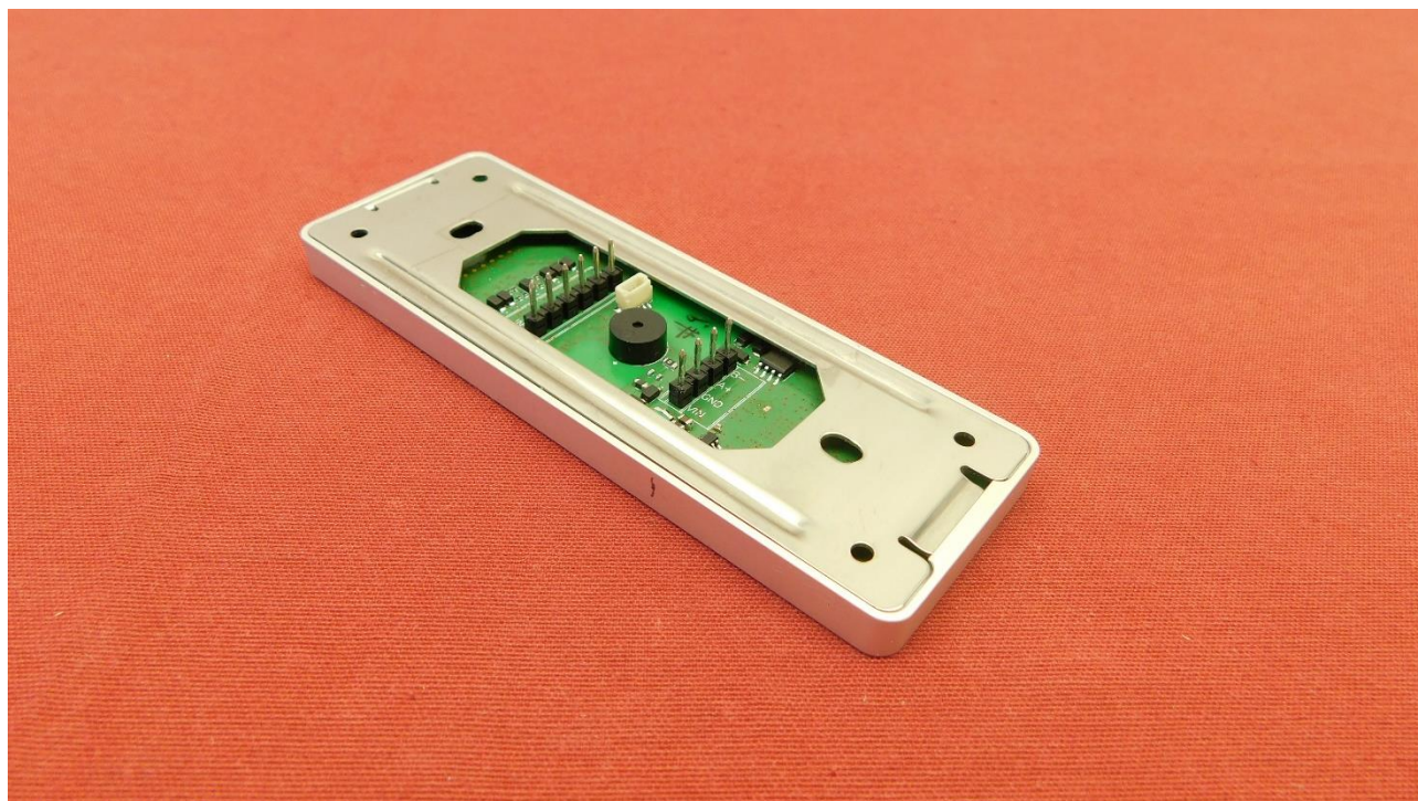
Picture 3: EUT – rear view with mounting bracket
