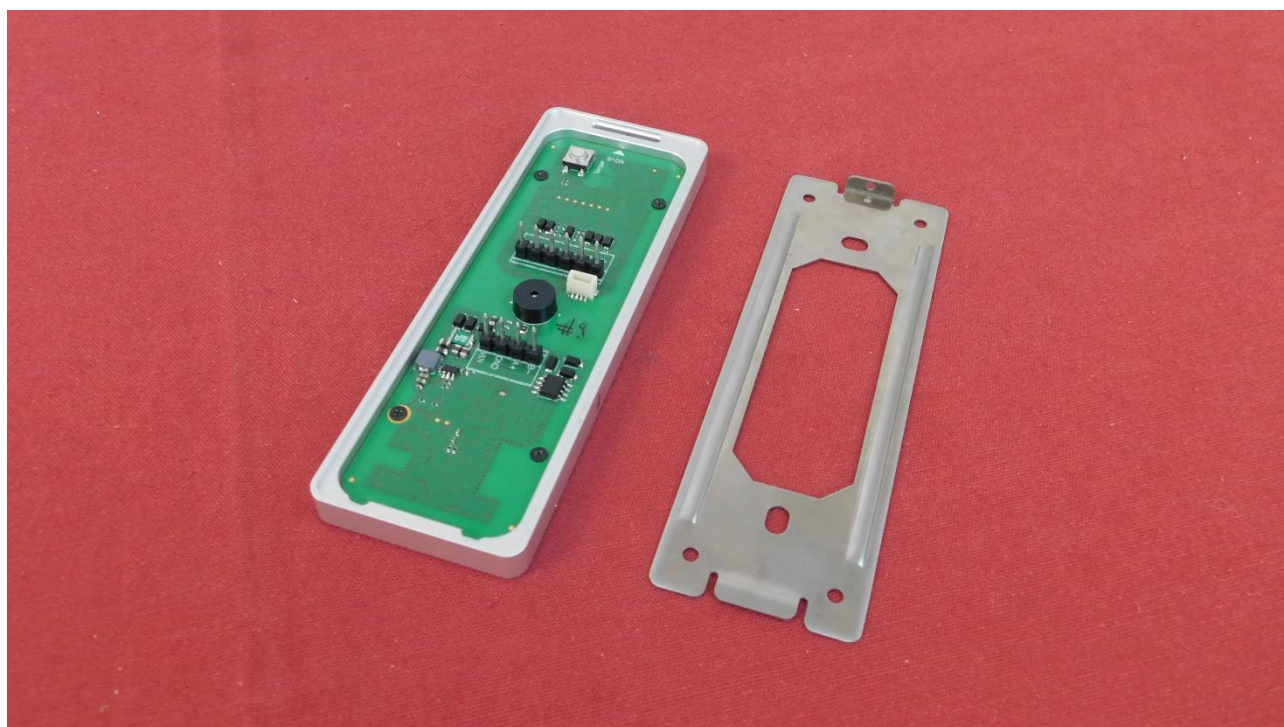
Picture 4: EUT – rear view with disassembled mounting bracket
