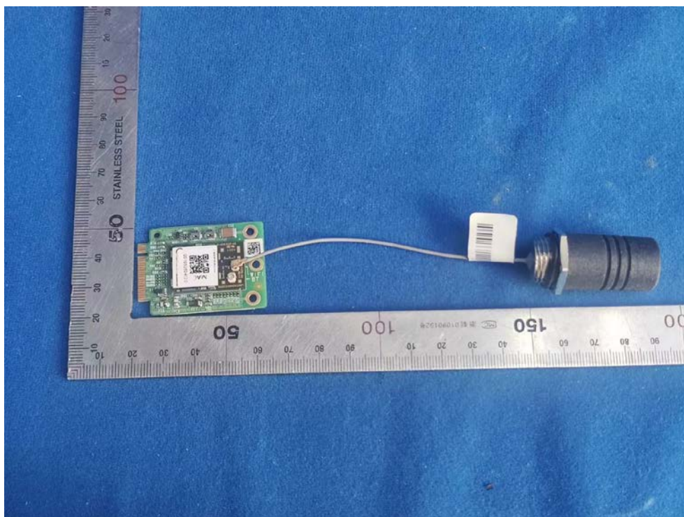
FIGURE 2 WIRELESS MODULE (MTxP250303ANT1) BACK VIEW
