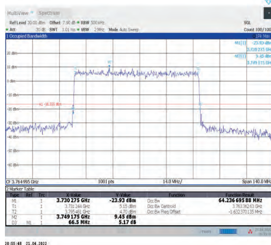
1-N78-3700-3800--30-70-H-5-DFT-256QAM-Outer_F ull-180@0-Ant1-64.237-66.500-≤70-PASS
