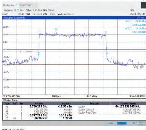
1-N78-3700-3800--30-70-H-2-DFT-PI2BPSK-Outer_F Full-180@0-Ant1-64.124-66.360-≤70-PASS
