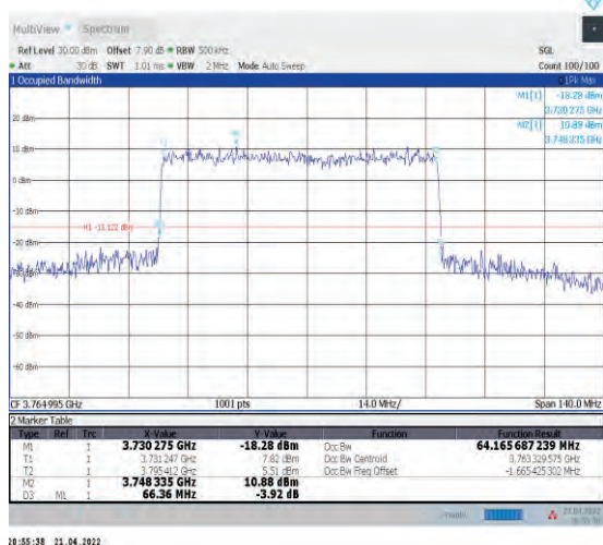
1-N78-3700-3800--30-70-H-4-DFT-64QAM-Outer_Fu ll-180@0-Ant1-64.166-66.360-≤70-PASS
