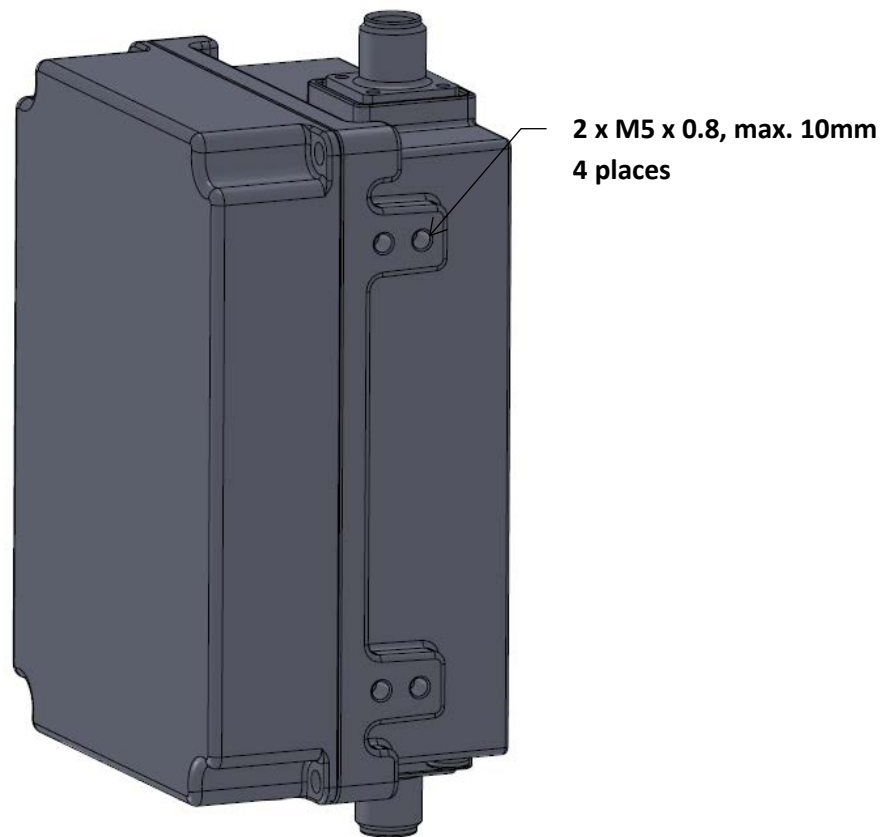
Figure 8: TTU Module Mounting Points
