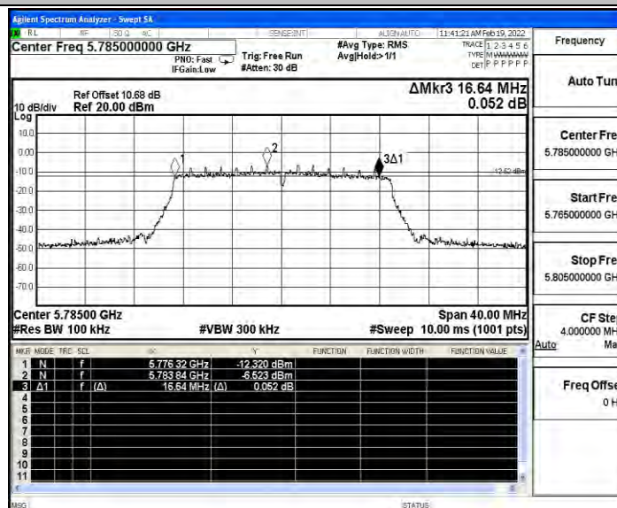
11N20SISO_Ant4_5785
