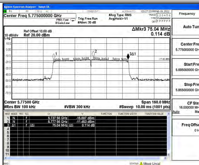
11AC80SISO_Ant6_5775
