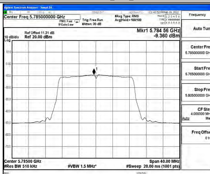
11AC20SISO_Ant7_5785
