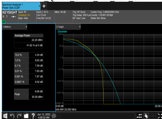
N78(20M)_DFT-s-OFDM QPSK Outer Full Low CH
