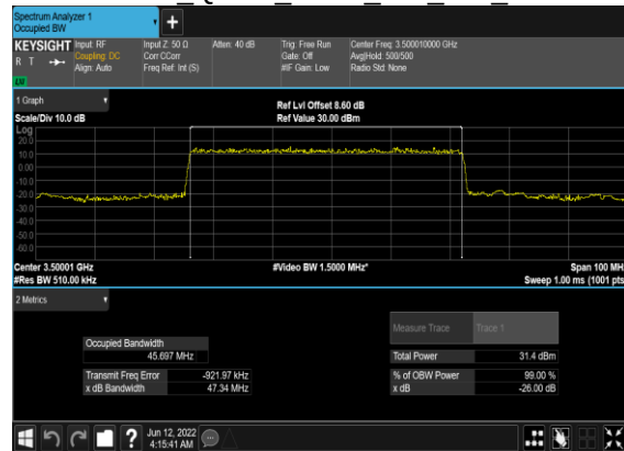
N78(50M)_DFT-s- OFDM QPSK Outer Full Mid CH
