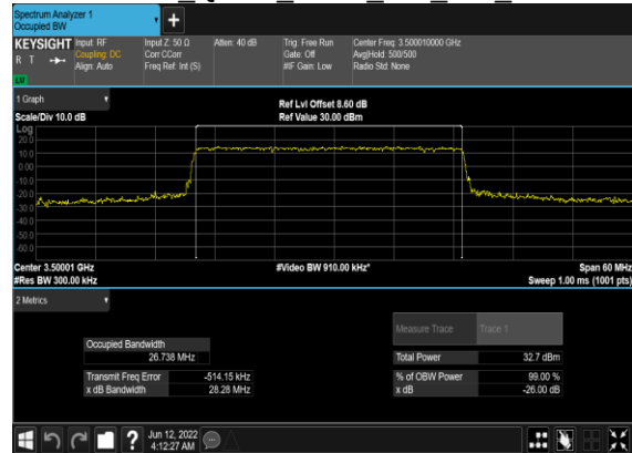
N78(30M)_DFT-s- OFDM QPSK Outer Full Mid CH
