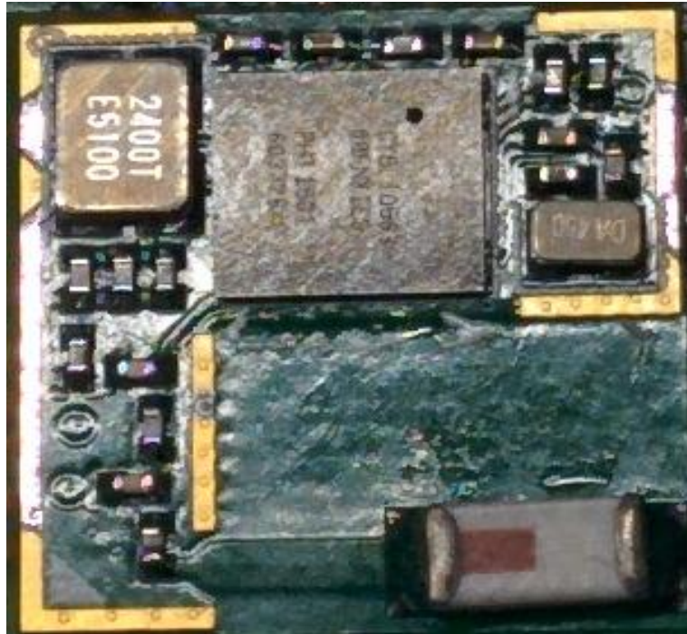
EUT Internal View - Shield removed
