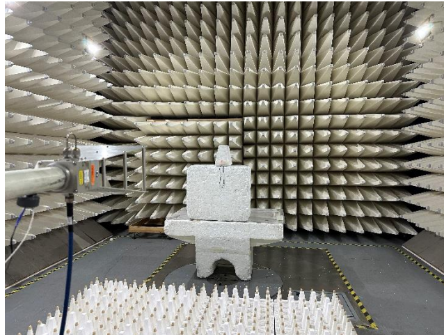
Photograph 1 Setup for OBW measurements
