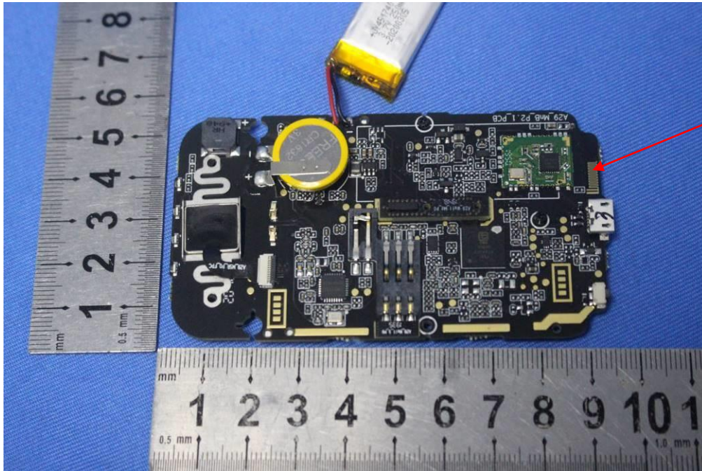
BT antenna
