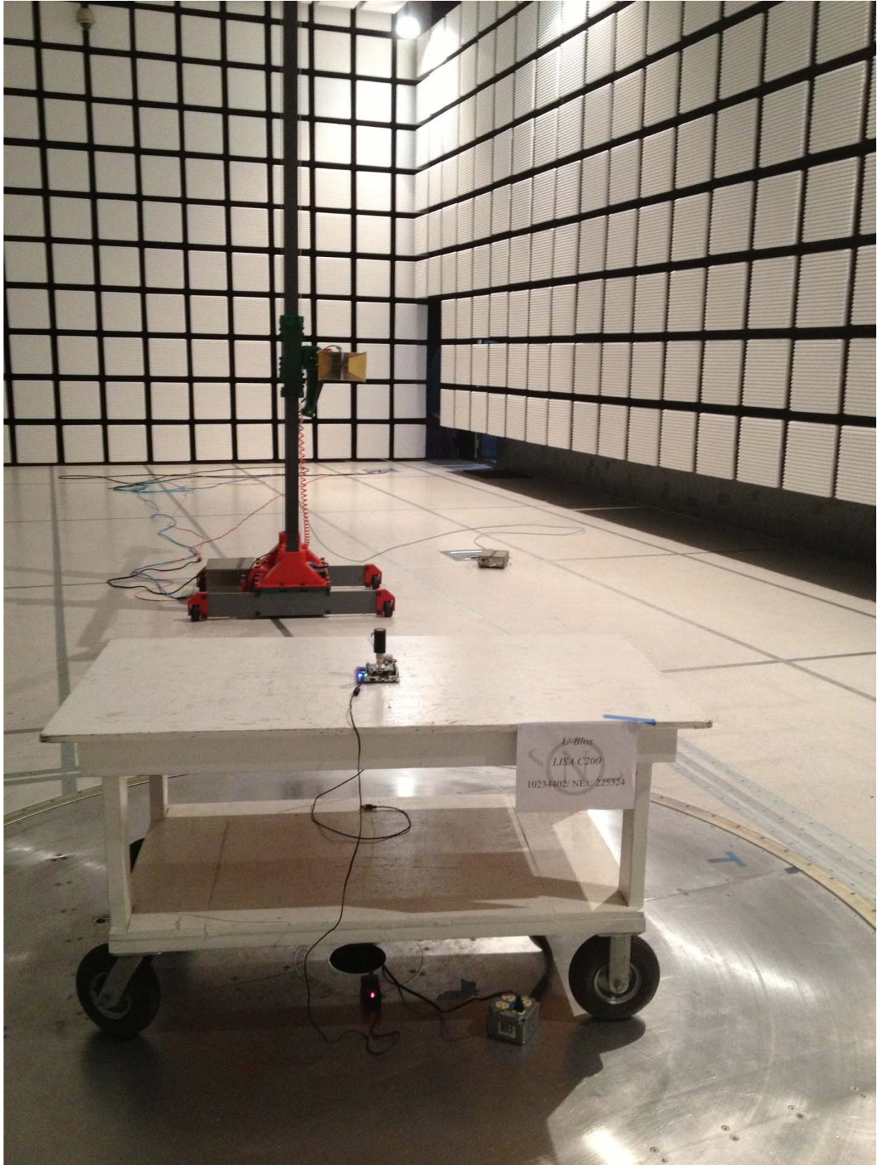
Radiated Field Strength Spurious Emission Test Setup
