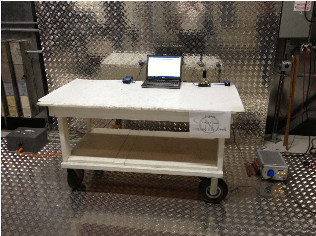
Conducted emissions on AC power line test setup
