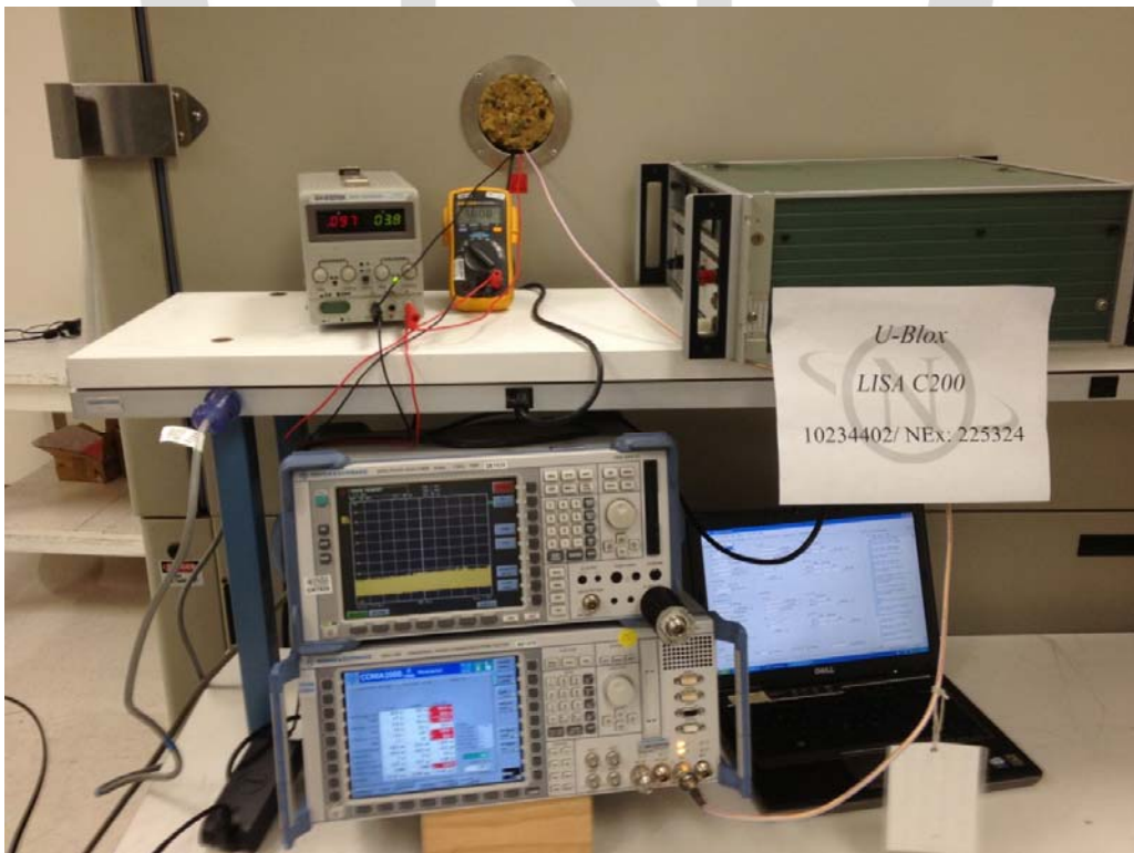
Frequency Stability set up
