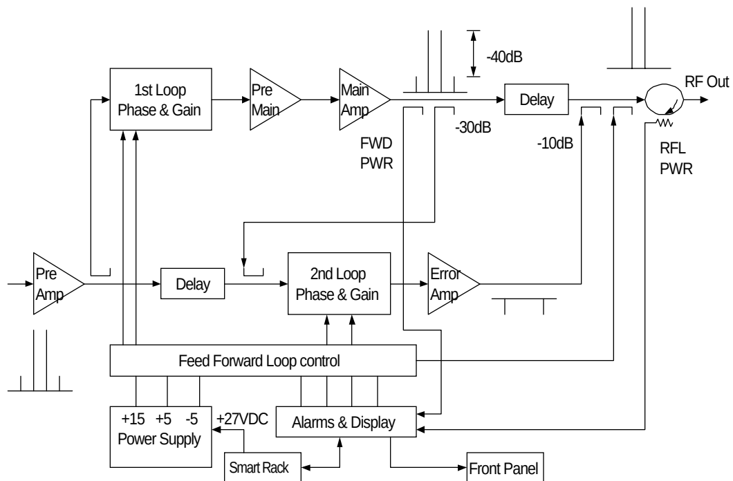
Multi-Carrier Power Amplifier Functional Block Diagram
