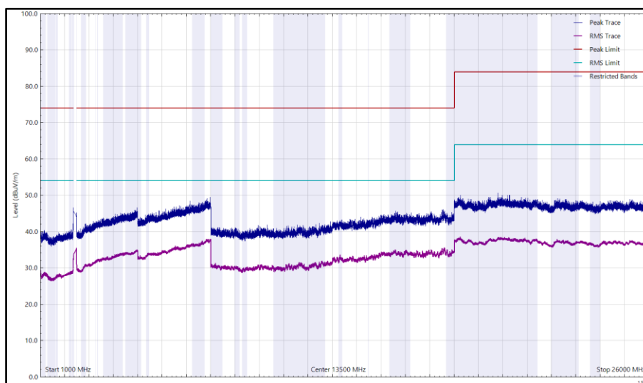
Figure 132 - 2412 MHz (CH1), HT20, CDD, Core 0 + Core 1, 1 GHz to 26 GHz, Vertical
