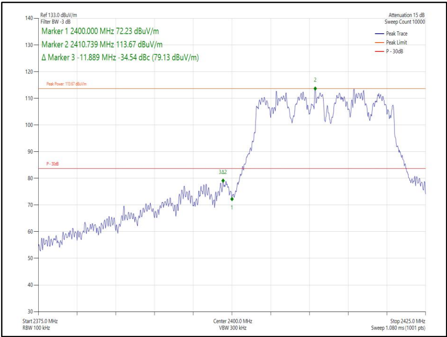
Figure 87 - 802.11n, HT20, CDD, Core 0-1 - 2412 MHz, Band Edge Frequency 2400 MHz
