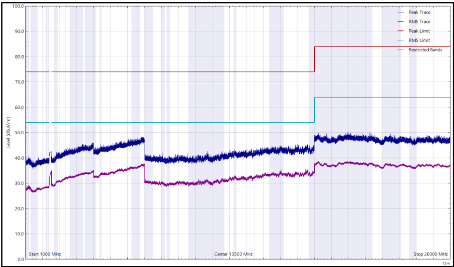
Figure 122 - 2472 MHz (CH13), 802.11b, Core 1, 1 GHz to 26 GHz, Vertical
