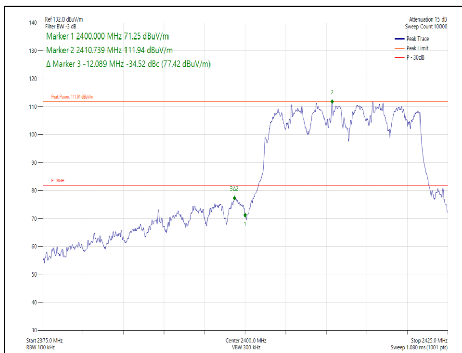
Figure 88 - 802.11ax, HE20, SU, CDD, Core 0-1 - 2412 MHz, Band Edge Frequency 2400 MHz
