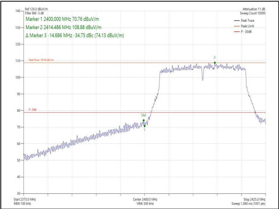
Figure 84 - 802.11n, HT20, SISO, Core 1 - 2412 MHz, Band Edge Frequency 2400 MHz
