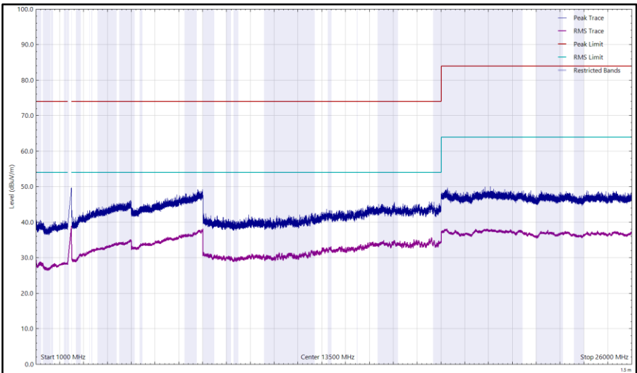
Figure 106 - 2437 MHz (CH6), 802.11g, Core 1, 1 GHz to 26 GHz, Vertical
