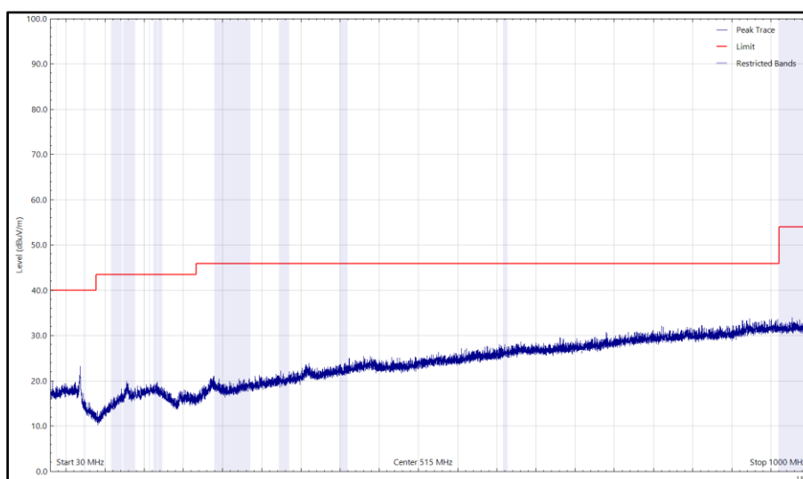
Figure 91 - 2437 MHz (CH6), 802.11b, Core 0, 30 MHz to 1 GHz, Horizontal (Peak)
