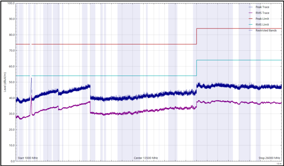
Figure 110 - 2437 MHz (CH6), HT20, CDD, Core 0 + Core 1, 1 GHz to 26 GHz, Vertical
