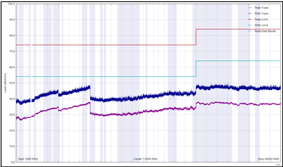
Figure 127 - 2412 MHz (CH1), 802.11g, Core 1, 1 GHz to 26 GHz, Horizontal
