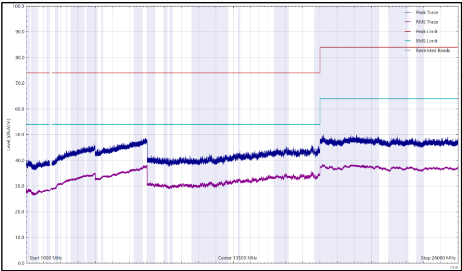
Figure 115 - 2412 MHz (CH1), 802.11b, Core 0, 1 GHz to 26 GHz, Horizontal
