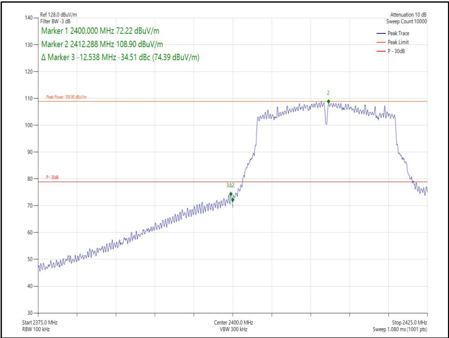
Figure 79 - 802.11n, HT20, SISO, Core 0 - 2412 MHz, Band Edge Frequency 2400 MHz
