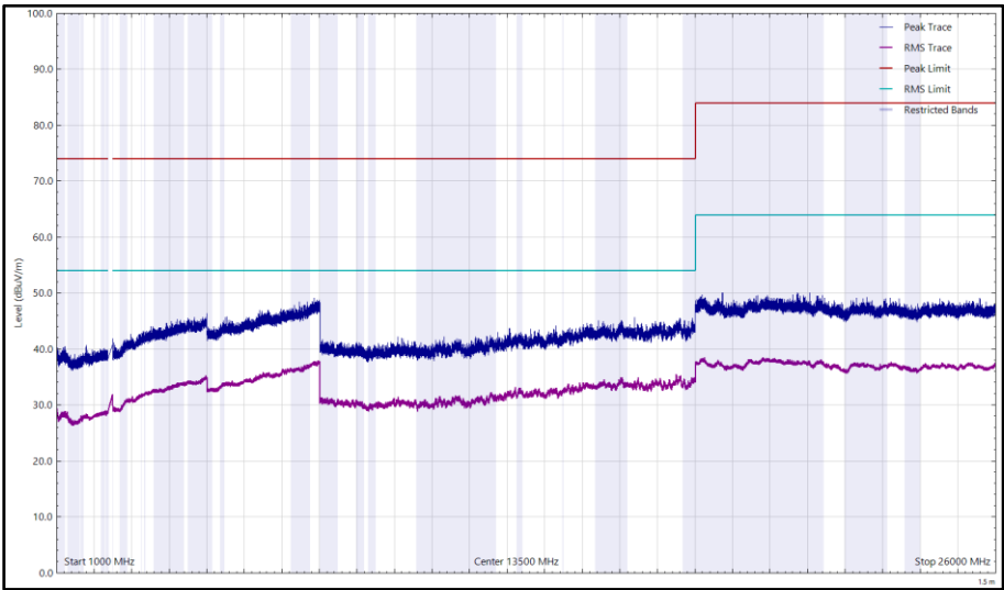
Figure 116 - 2412 MHz (CH1), 802.11b, Core 0, 1 GHz to 26 GHz, Vertical
