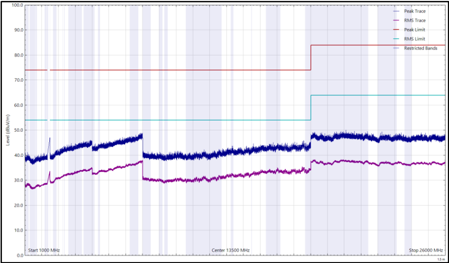
Figure 94 - 2437 MHz (CH6), 802.11b, Core 0, 1 GHz to 26 GHz, Vertical
