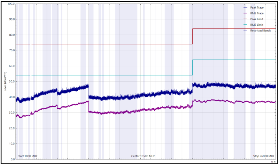
Figure 121 - 2472 MHz (CH13), 802.11b, Core 1, 1 GHz to 26 GHz, Horizontal
