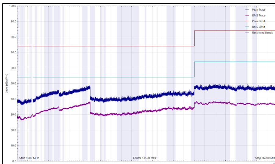
Figure 131 - 2412 MHz (CH1), HT20, CDD, Core 0 + Core 1, 1 GHz to 26 GHz, Horizontal
