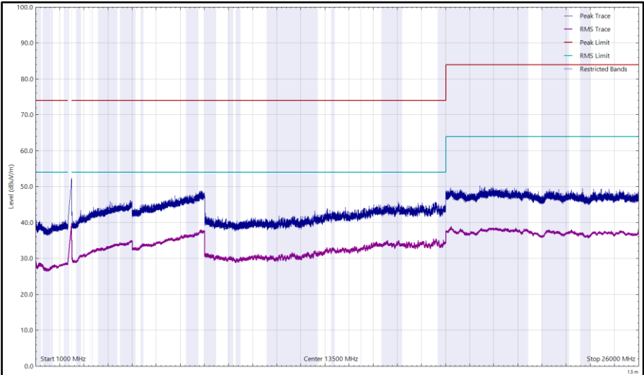
Figure 102 - 2437 MHz (CH6), 802.11g, Core 0, 1 GHz to 26 GHz, Vertical
