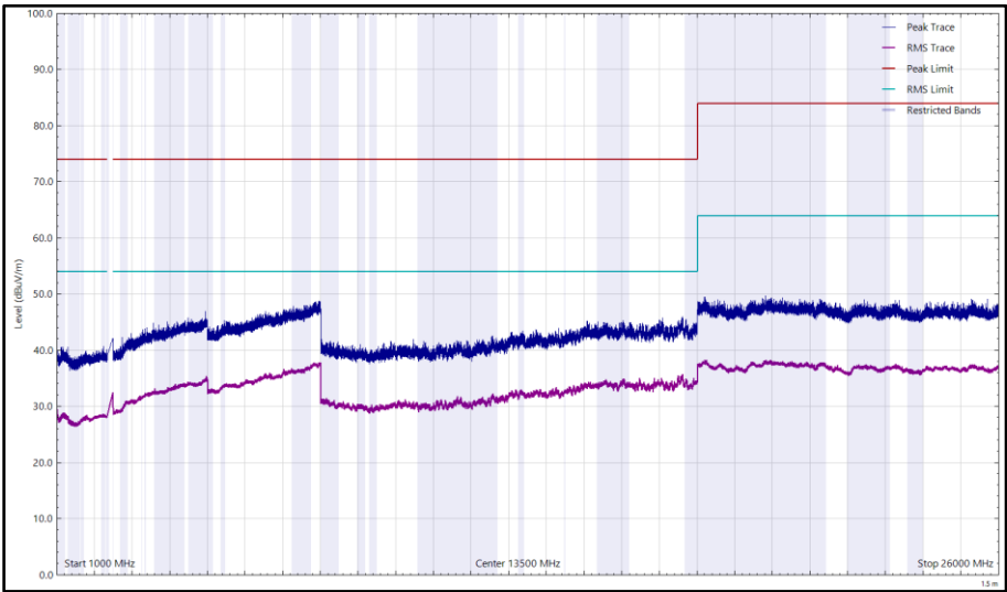
Figure 104 - 2437 MHz (CH6), 802.11g, Core 1, 1 GHz to 26 GHz, Horizontal
