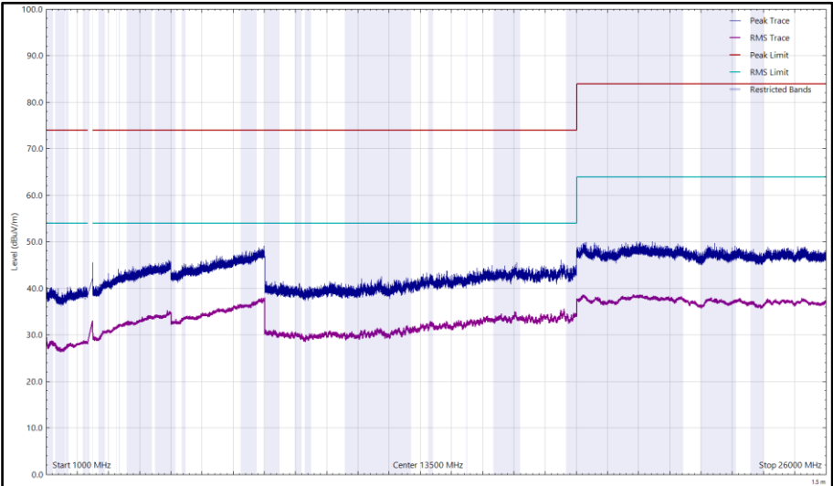
Figure 98 - 2437 MHz (CH6), 802.11b, Core 1, 1 GHz to 26 GHz, Vertical
