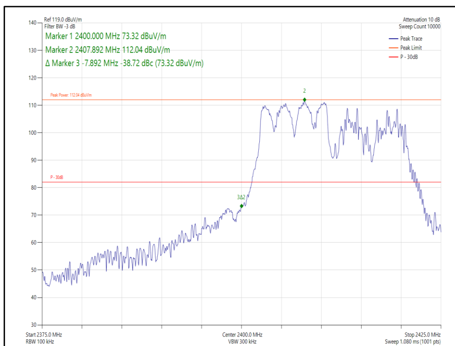
Figure 89 - 802.11ax, HE20, RU 106-53, CDD Core 0-1 - 2412 MHz, Band Edge Frequency 2400 MHz
