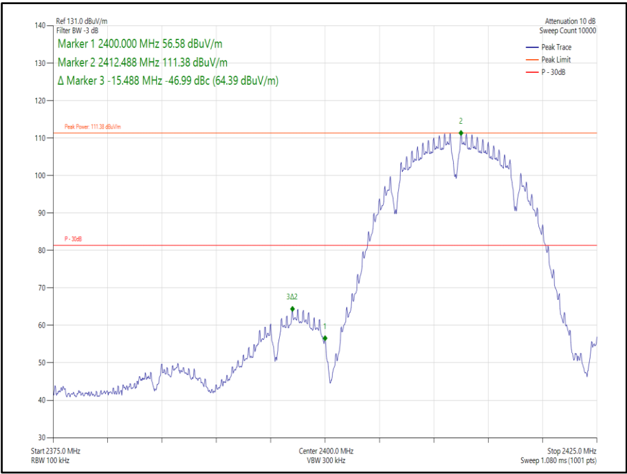
Figure 77 - 802.11b, SISO, Core 0 - 2412 MHz, Band Edge Frequency 2400 MHz
