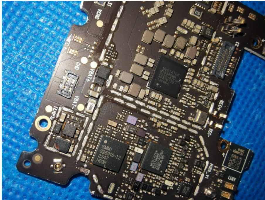
INTERNAL VIEW OF EUT(Figure 4)
