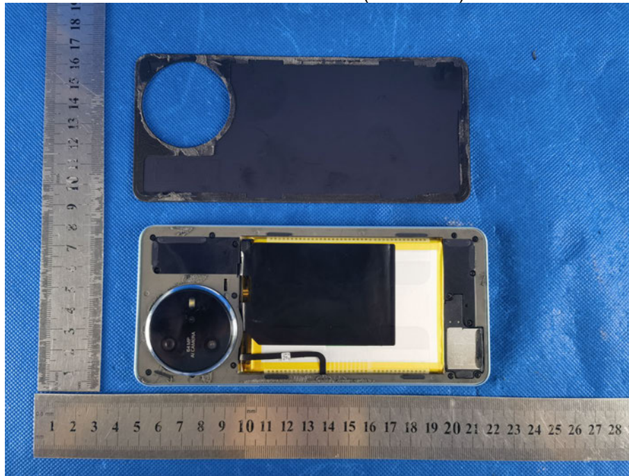
OPEN VIEW OF EUT(FIGURE 1)
