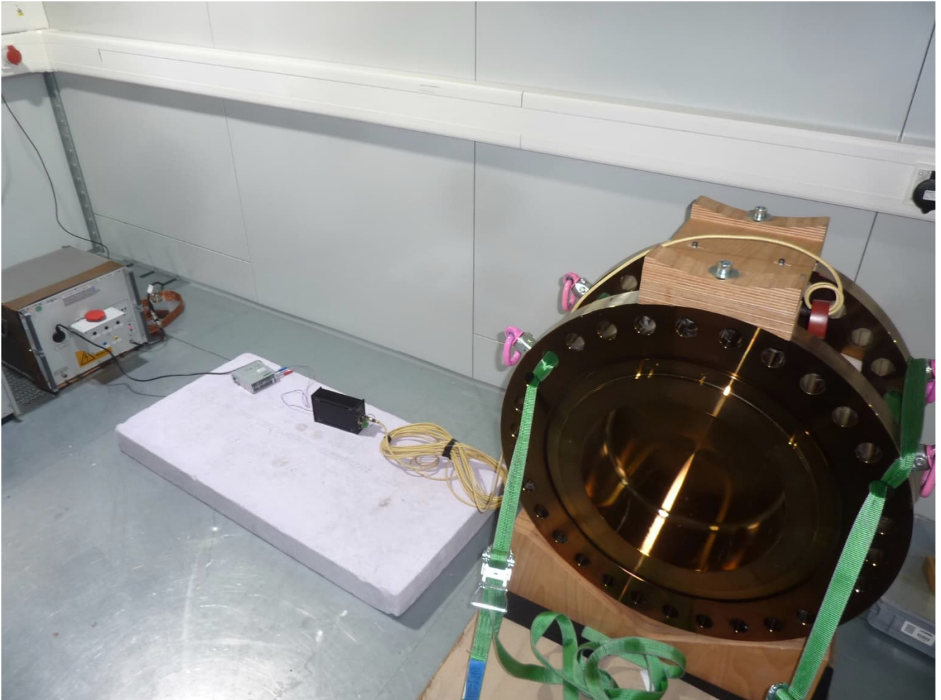
Setup 150 kHz to 30 MHz conducted emission measurement
