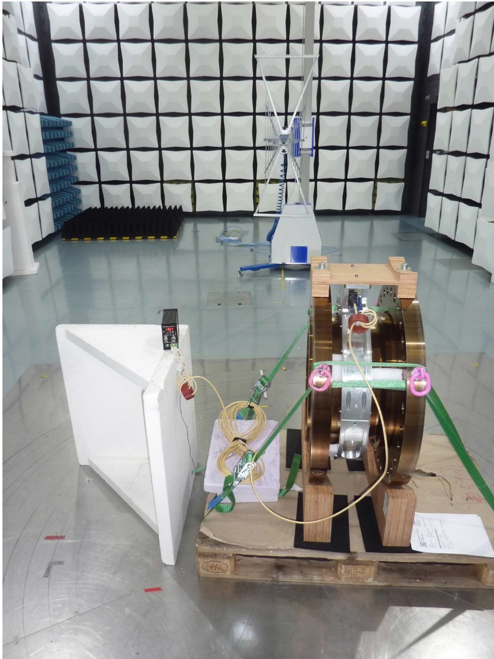
Setup 30 MHz to 1000 MHz radiated field strength measurement
