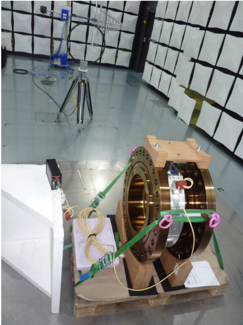
Setup 9 kHz to 30 MHz magnetic field strength preliminary measurement
