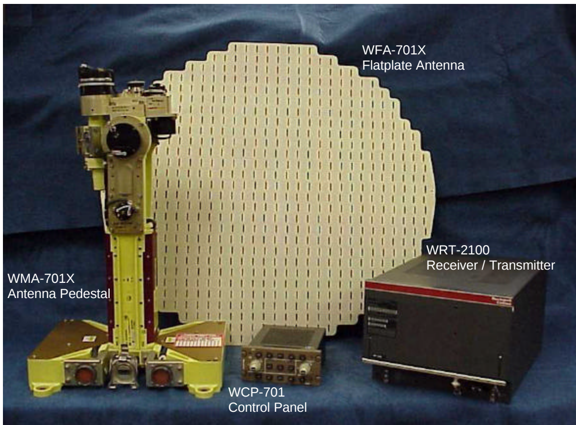
Figure C-1. WXR-2100 Family
