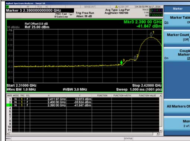
2412 MHz – Peak
