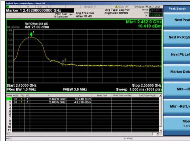
2462 MHz – Peak
