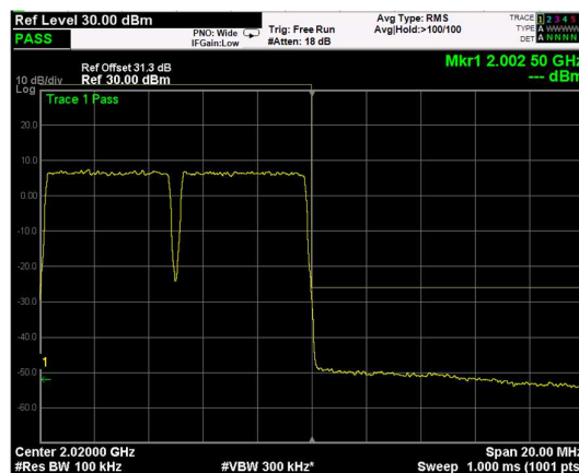
High Band Edge, 2 Carrier, Modulation: QPSK, BW=5MHz
