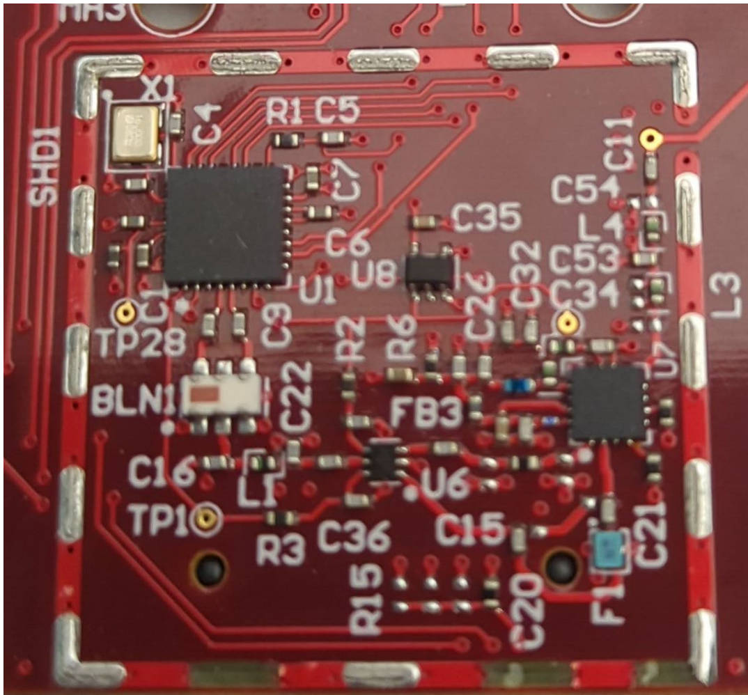
Close Up of RF Section
