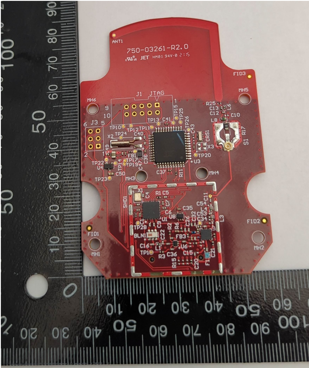
Shield Removed
