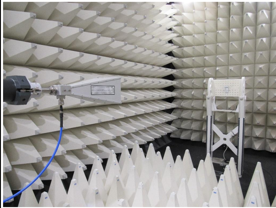
Test Setup radiated emissions transmit mode above 1 GHz
