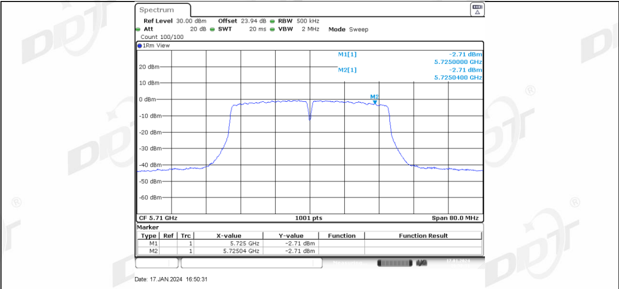
11AC40MIMO Ant2 5710 UNII-3
