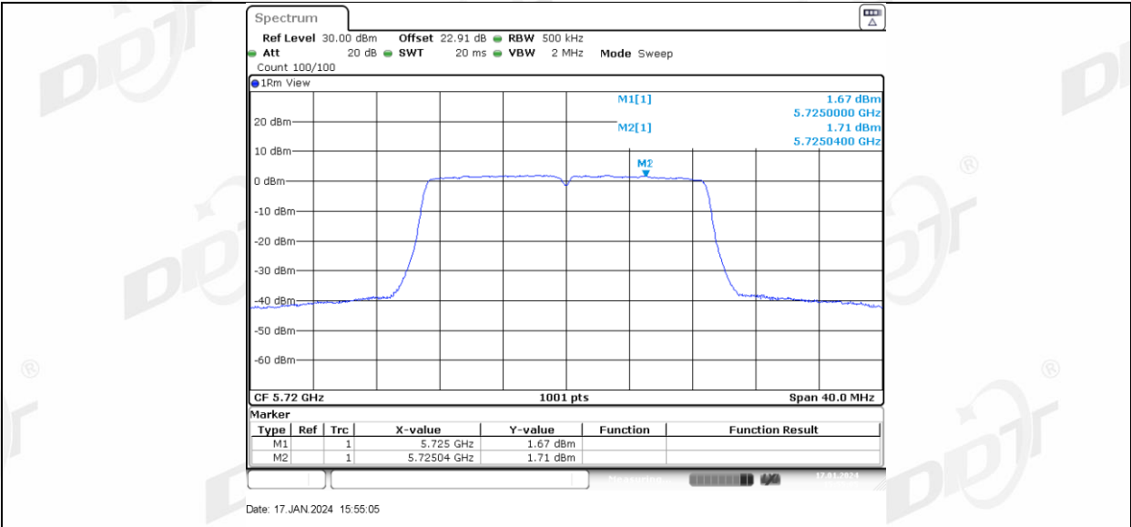
11AC20MIMO Ant2 5720 UNII-3
