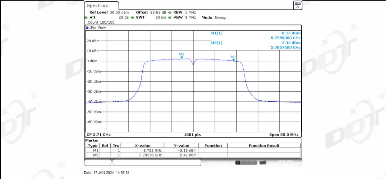
11N40MIMO Ant2 5710 UNII-2C
