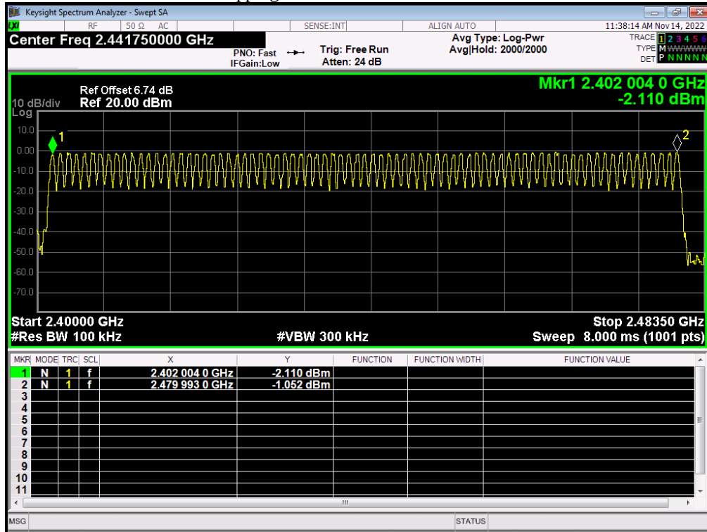
Hopping No. NVNT 1-DH5 2441MHz
