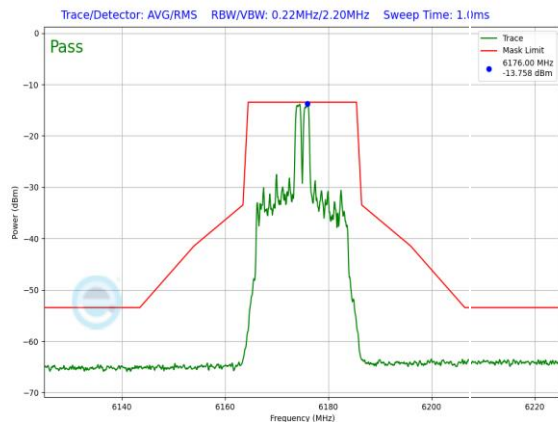
Plot 7-1411. LPI In-Band Emission Plot SDM Diversity Antenna WF7a (20MHz 802.11ax RU26 (UNII Band 5) – Ch. 45)
