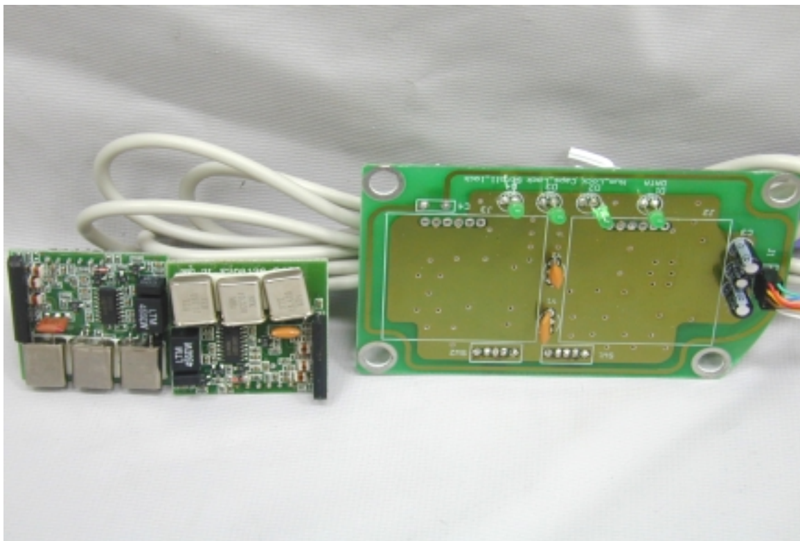
PHOTO. 6. EUT (RX Model CKM001) COMPONENT SIDE VIEW
