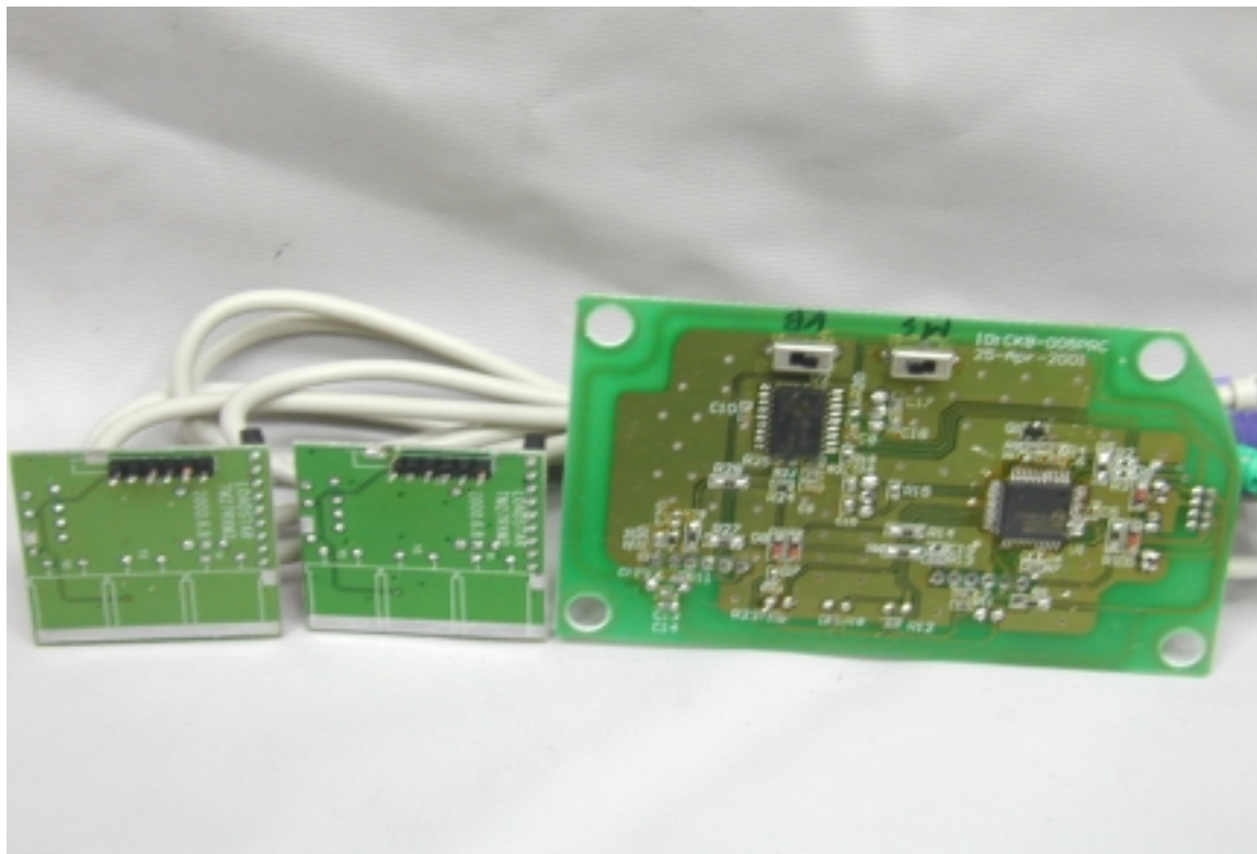
PHOTO. 7. EUT (RX Model CKM001) SOLDERING SIDE VIEW
