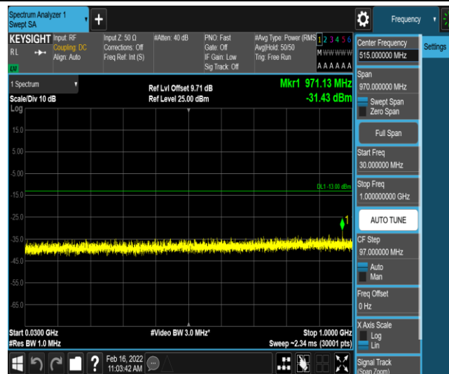
Band66-10MHz-16QAM-132622-1-0-High-30-1000--31.43-PASS
