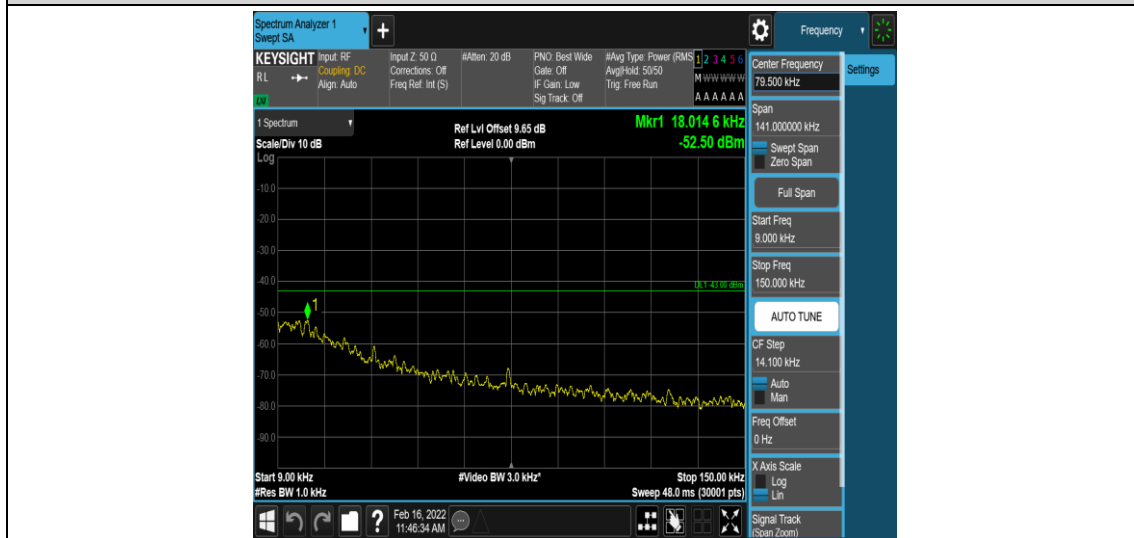
Band66-20MHz-QPSK-132322-1-0-Low-0.009-0.15--52.5-PASS
