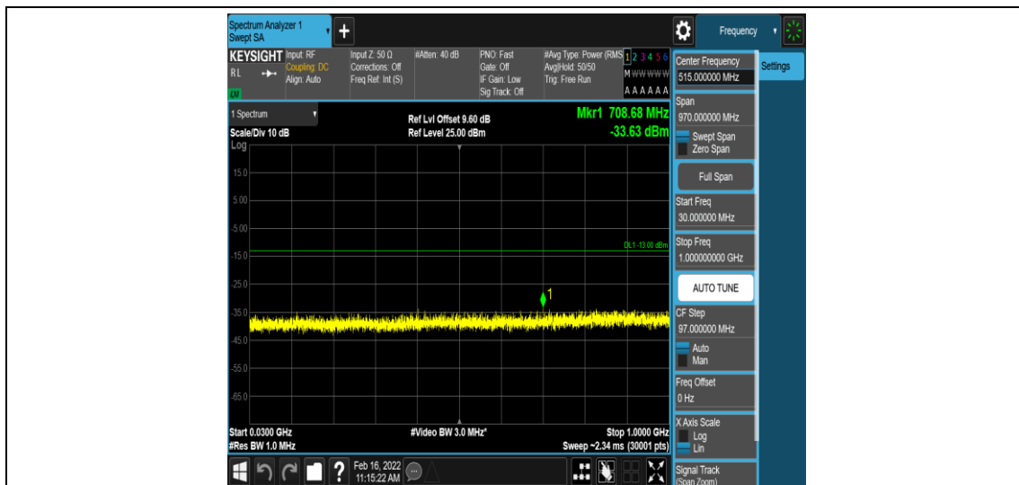
Band66-15MHz-16QAM-132047-1-0-Low-30-1000--33.63-PASS
