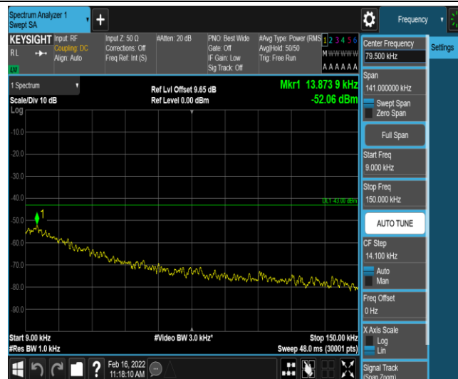
Band66-15MHz-16QAM-132322-1-0-Low-0.009-0.15--52.06-PASS
