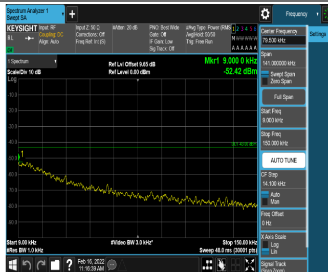
Band66-15MHz-QPSK-132322-1-0-Low-0.009-0.15--52.42-PASS
