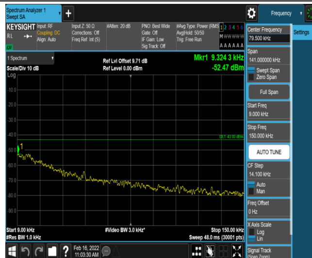
Band66-10MHz-16QAM-132622-1-0-High-0.009-0.15--52.47-PASS
