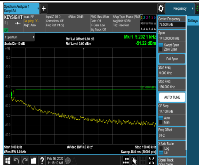
Band66-15MHz-16QAM-132047-1-0-Low-0.009-0.15--51.22-PASS
