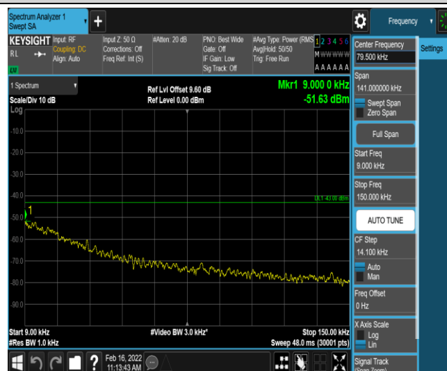
Band66-15MHz-QPSK-132047-1-0-Low-0.009-0.15--51.63-PASS
