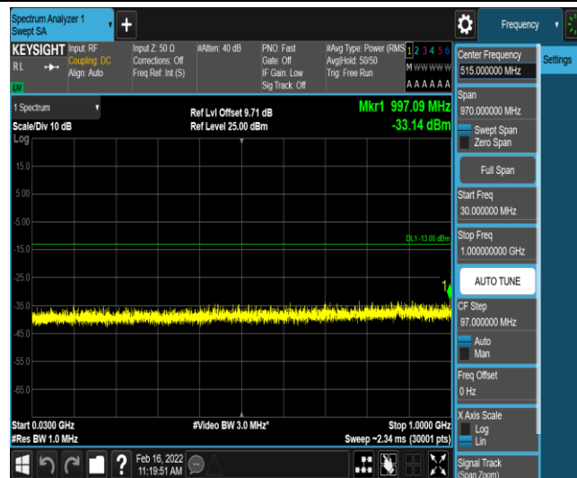
Band66-15MHz-QPSK-132597-1-0-High-30-1000--33.14-PASS
