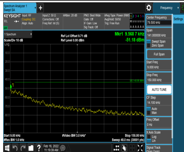
Band66-15MHz-QPSK-132597-1-0-High-0.009-0.15--51.19-PASS
