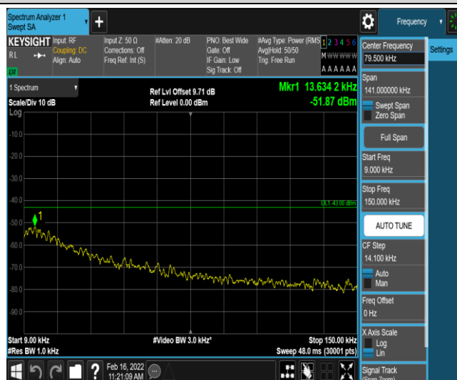
Band66-15MHz-16QAM-132597-1-0-High-0.009-0.15--51.88-PASS
