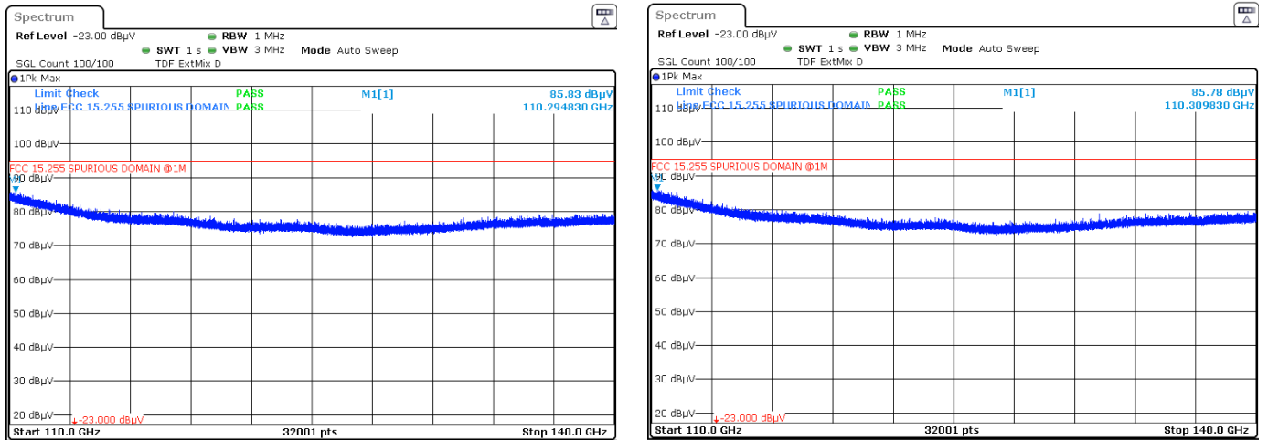
Figure 7.3-8: Unwanted emissions spurious band plot @1m – Field strength measured from 110 to 140 GHz, horizontal and vertical polarization respectively.
