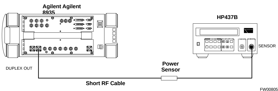
Figure H-6: Delta Calibration Setup - Agilent 8935 to HP437
