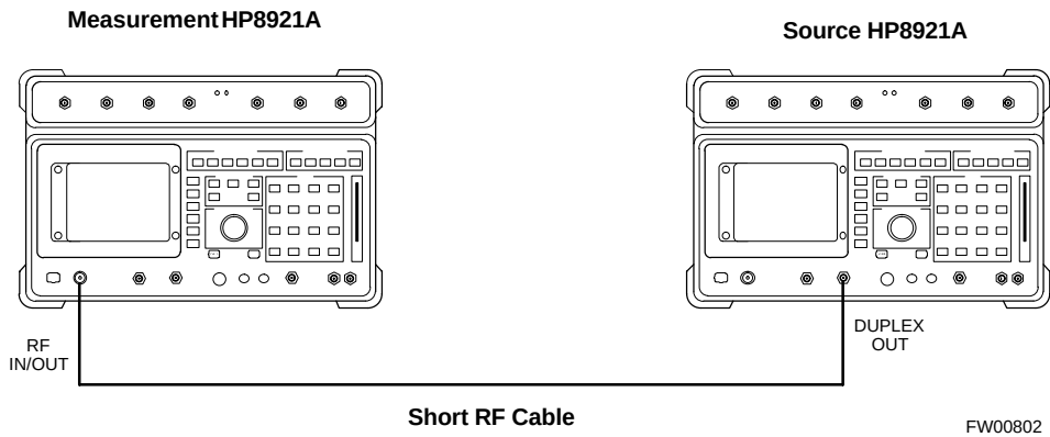
Figure H-9: Delta Calibration Setup - HP8921A to HP8921A
