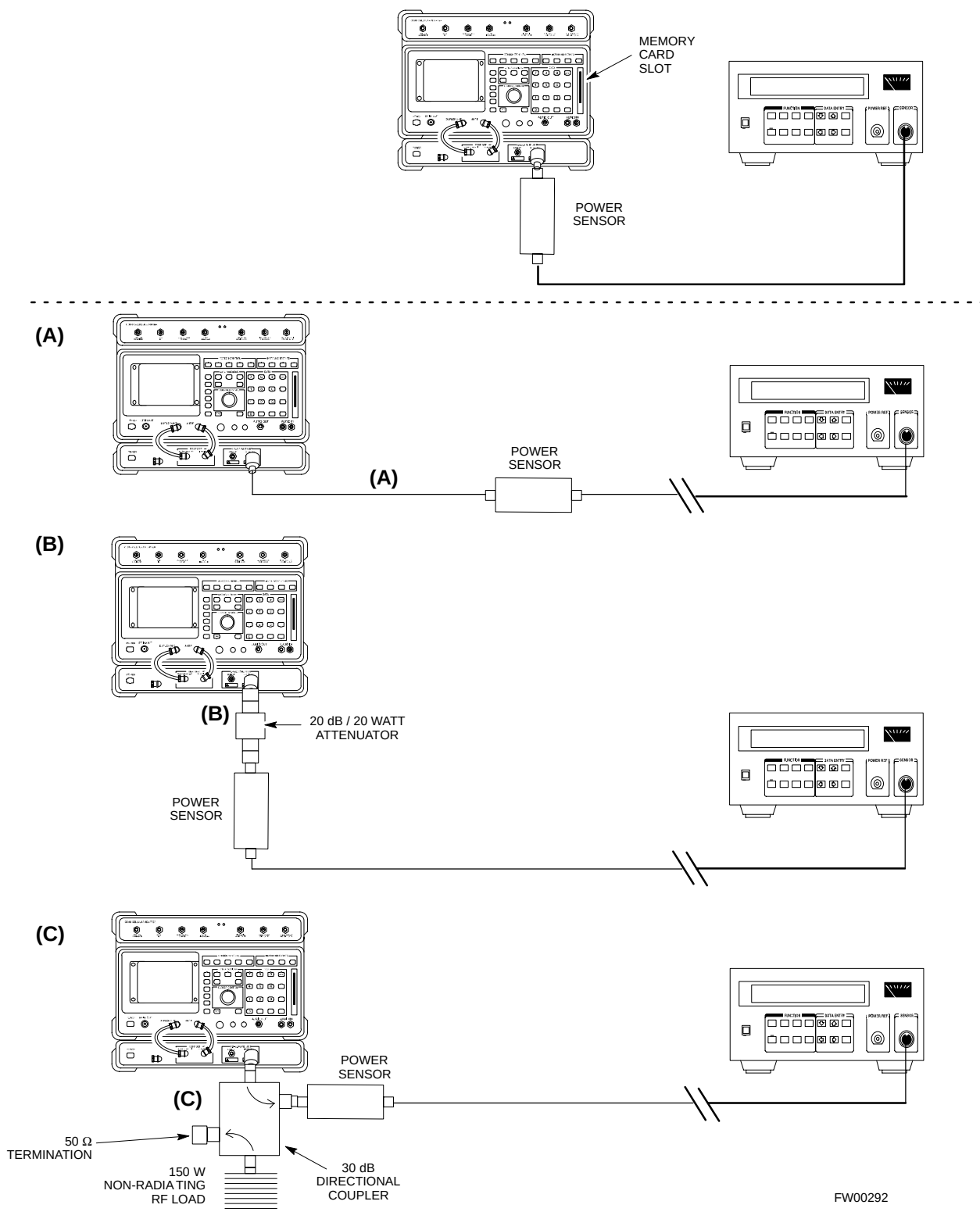
Figure F-21: Cable Calibration Using HP8921 with PCS Interface
