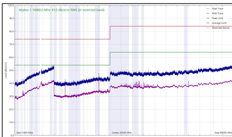
Figure 9 - U-NII-2C - 5640 MHz (CH128), VHT20, CDD, Core 0 + Core 1 and 2441 MHz (CH39), 2-DH5, ePA, Core 0 + Core 1, 1 GHz to 40 GHz, Vertical
