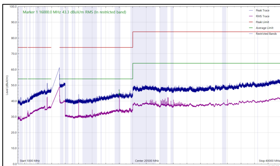
Figure 21 - U-NII-8 - 7115 MHz (CH233), HE20, SU, CDD, Core 0 + Core 1 and 2441 MHz (CH39), 2-DH5, ePA, Core 0 + Core 1, 1 GHz to 40 GHz, Vertical
