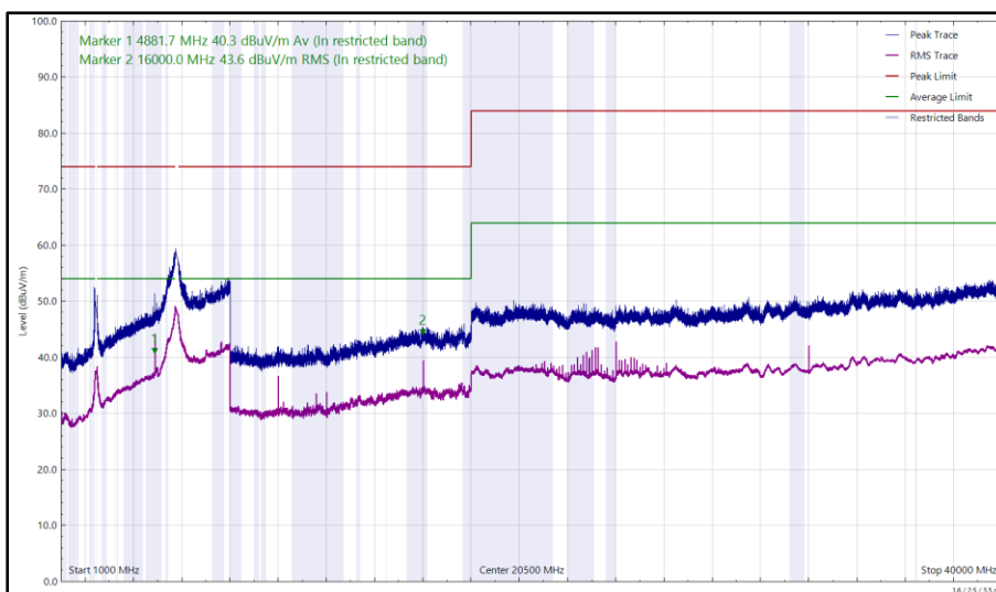
Figure 11 - U-NII-3 - 5785 MHz (CH157), VHT20, CDD, Core 0 + Core 1 and 2441 MHz (CH39), 2-DH5, ePA, Core 0 + Core 1, 1 GHz to 40 GHz, Horizontal
