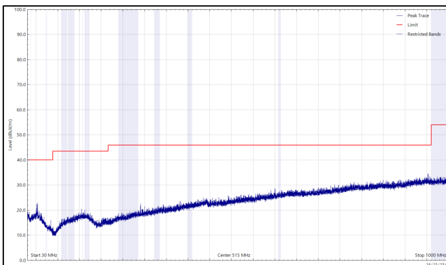
Figure 10 - U-NII-3 - 5785 MHz (CH157), VHT20, CDD, Core 0 + Core 1 and 2441 MHz (CH39), 2-DH5, ePA, Core 0 + Core 1, 30 MHz to 1 GHz, Horizontal (Peak)
