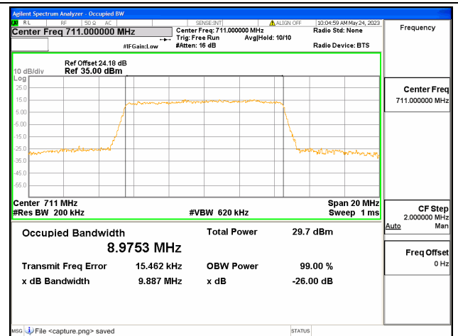
Band17 / 10MHz / 64QAM/ High CH
