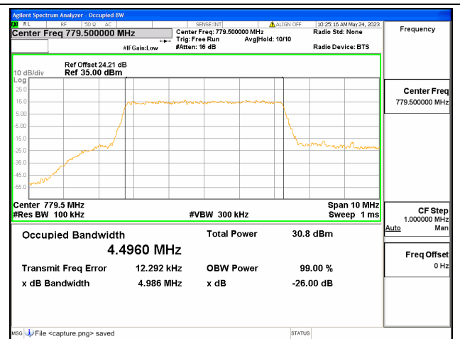
Band13 / 5MHz / 16QAM/ Low CH
