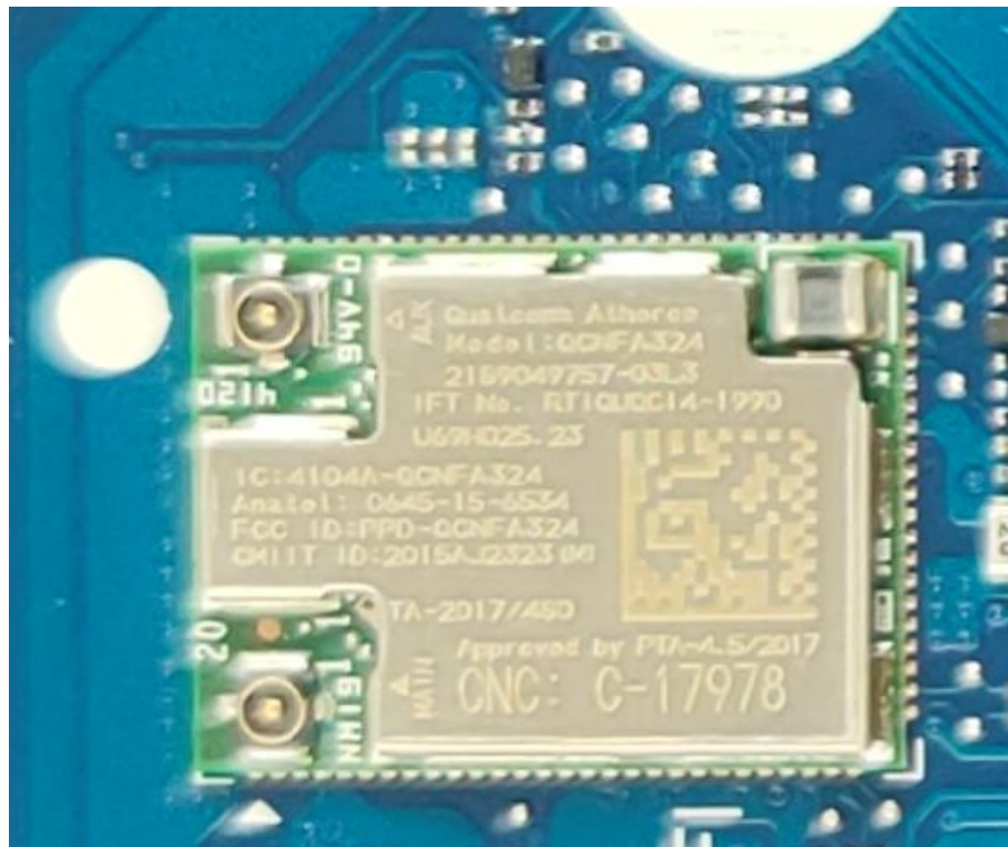
RF MODULE TOP VIEW
