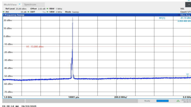
Band4-10MHz-QPSK-20175-1RB#49-1000~3000-PASS
