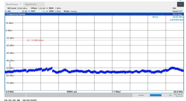
Band4-10MHz-QPSK-20175-1RB#49-3000~20000-PASS
