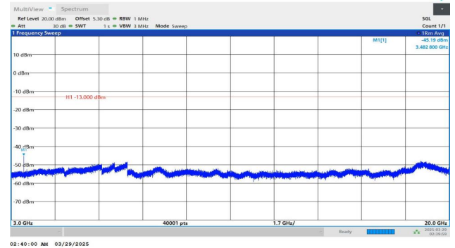
Band4-20MHz-QPSK-20175-1RB#99-3000~20000-PASS
