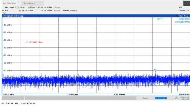
Band4-20MHz-QPSK-20175-1RB#99-0.15~30-PASS
