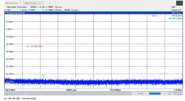
Band4-20MHz-QPSK-20175-1RB#99-30~1000-PASS
