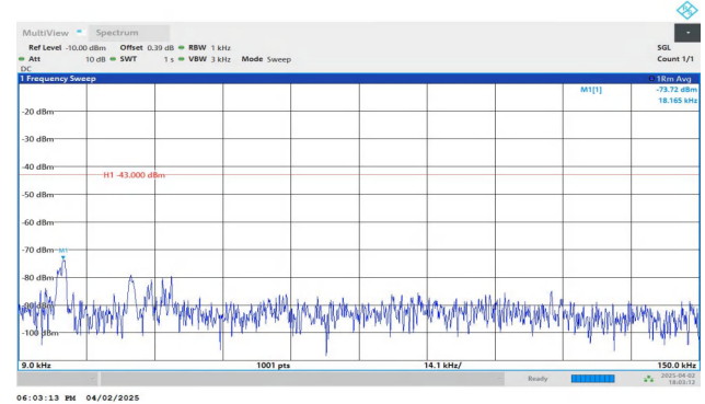
Band4-10MHz-QPSK-20350-1RB#49-0.009~0.15-PASS
