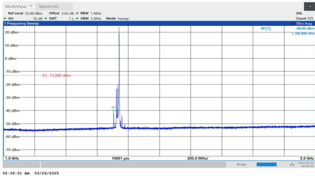
Band4-20MHz-QPSK-20175-1RB#99-1000~3000-PASS
