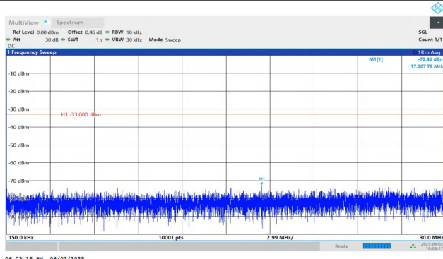
Band4-10MHz-QPSK-20350-1RB#49-0.15~30-PASS
