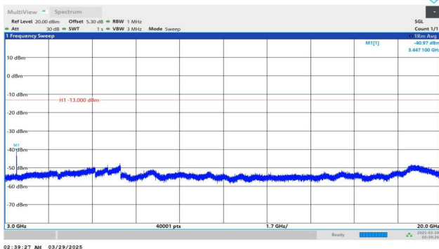
Band4-20MHz-QPSK-20175-1RB#0-3000~20000-PASS
