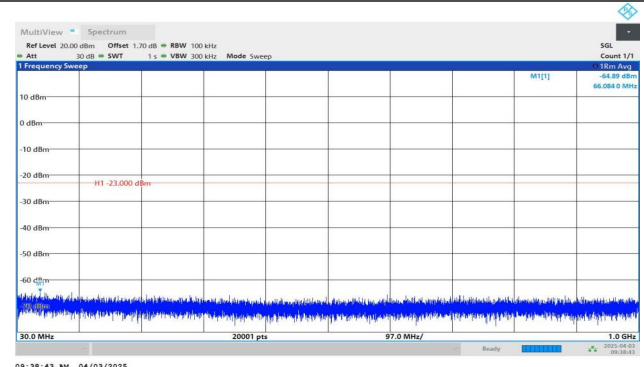
Band4-10MHz-QPSK-20350-1RB#49-30~1000-PASS
