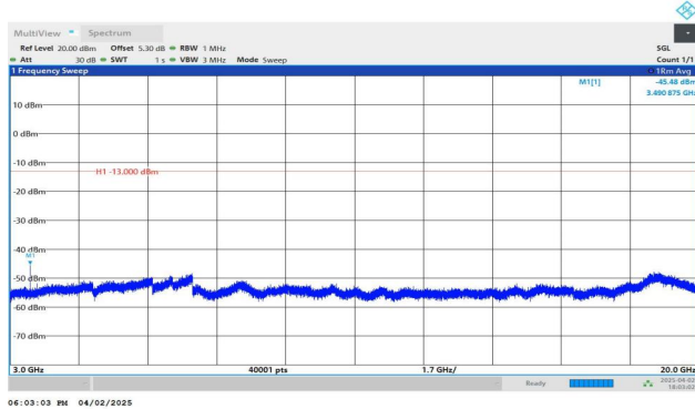
Band4-10MHz-QPSK-20350-1RB#0-3000~20000-PASS
