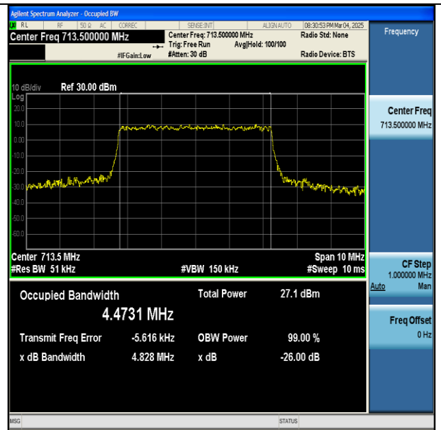
NTNV-n12-PC3-15-5-H-CP-64QAM-Outer_Full-Ant1-PASS
