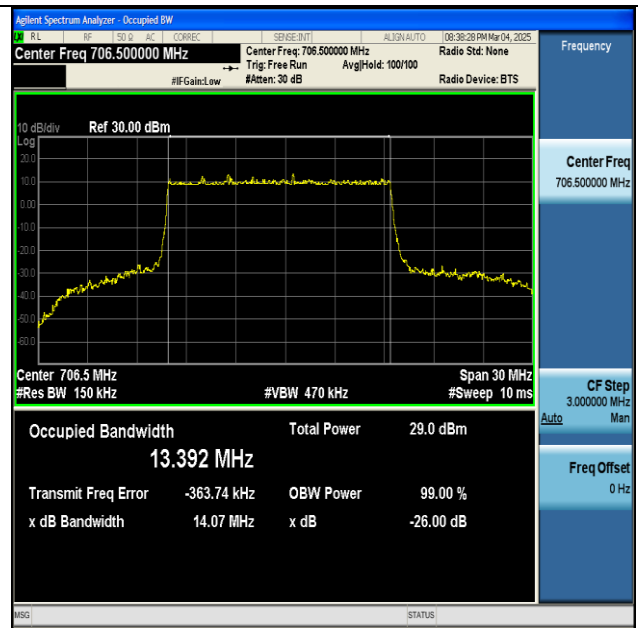
NTNV-n12-PC3-15-15-L-DFT-64QAM-Outer_Full-Ant1- PASS
