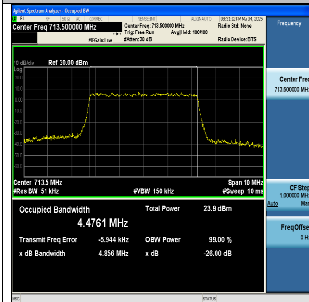
NTNV-n12-PC3-15-5-H-CP-256QAM-Outer_Full-Ant1- PASS
