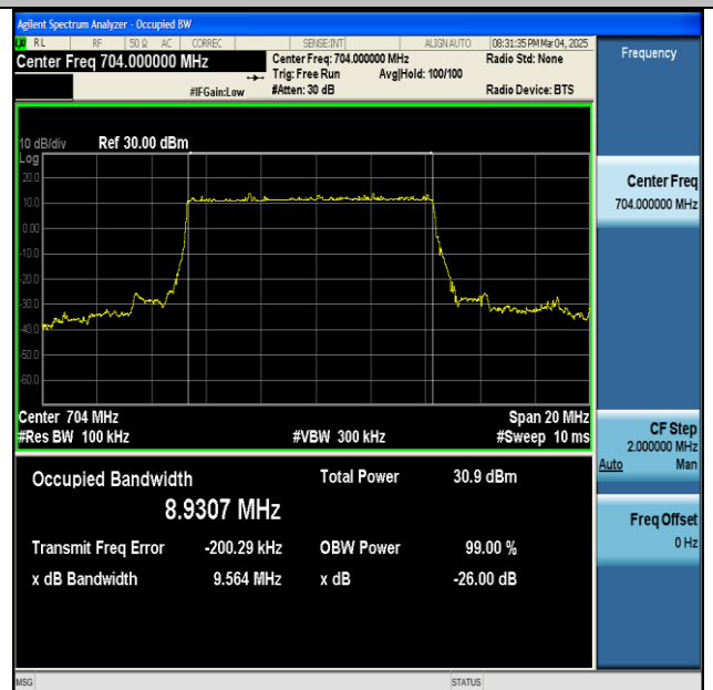
NTNV-n12-PC3-15-10-L-DFT-BPSK-Outer_Full-Ant1- PASS
