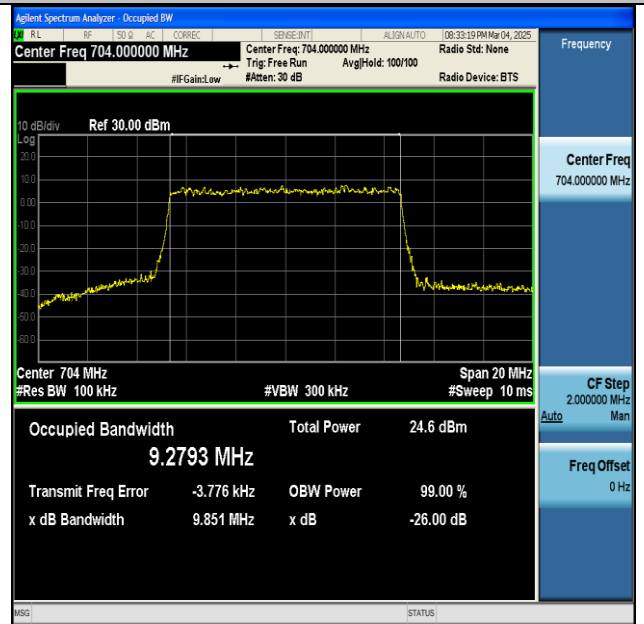
NTNV-n12-PC3-15-10-L-CP-256QAM-Outet_Full-Ant1-PASS
