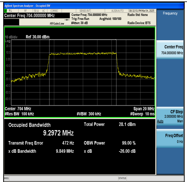
NTNV-n12-PC3-15-10-L-CP-16QAM-Outet_Full-Ant1-PASS
