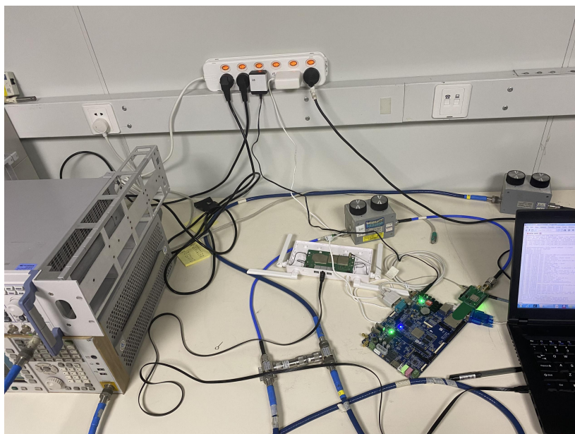
DFS Test setup
