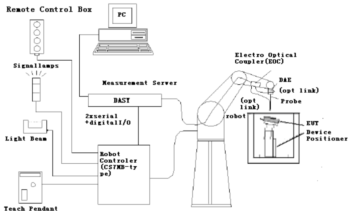
Figure 1 HAC Test Measurement Set-up
