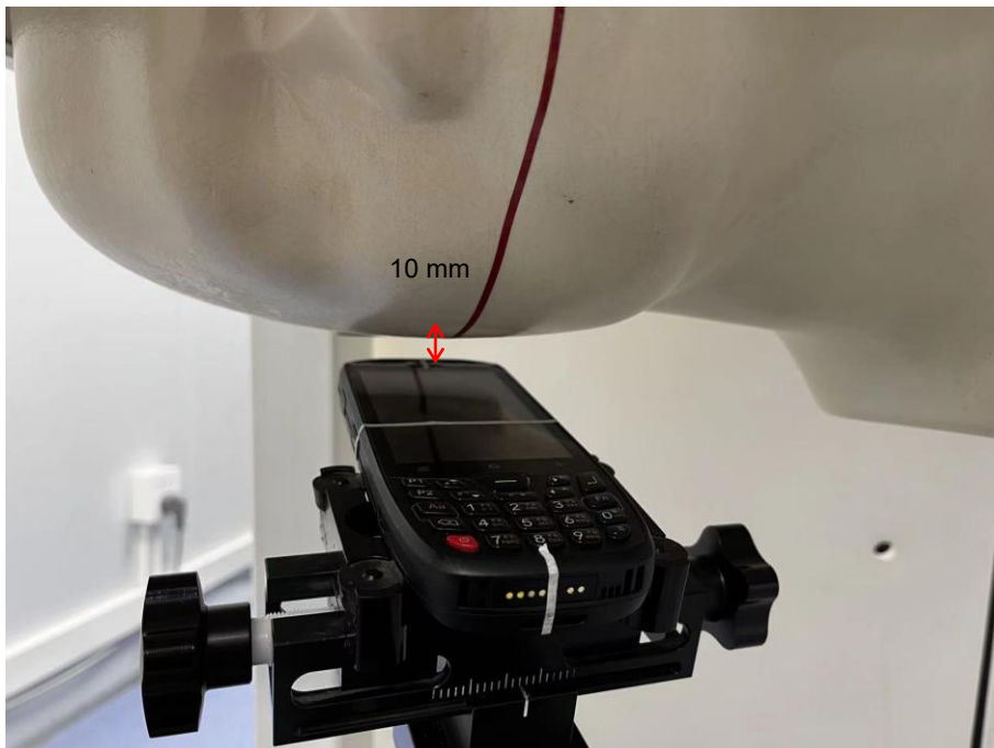
Right Head Tilt (15° ) (10mm)
