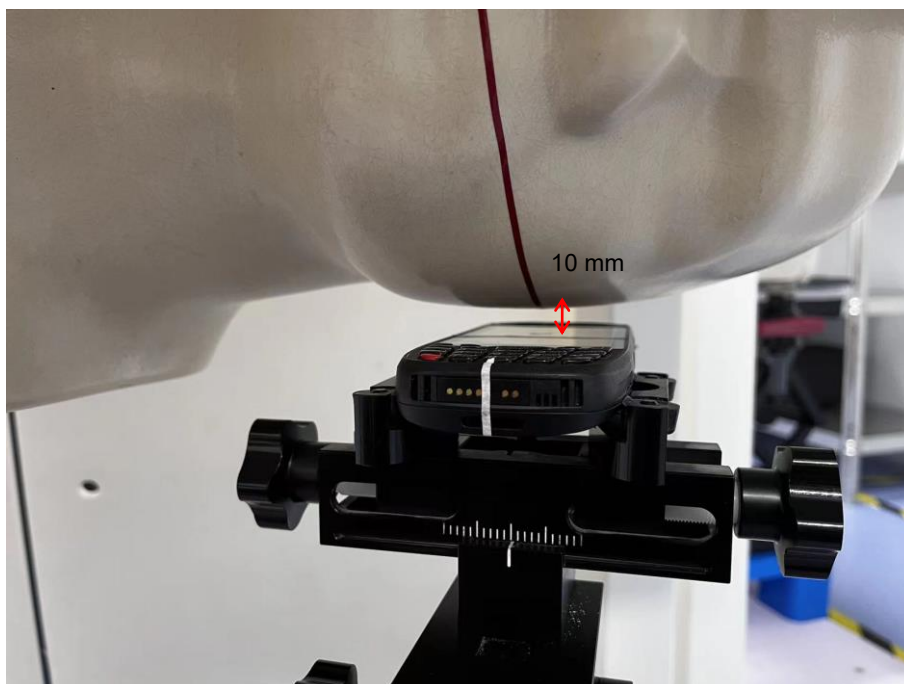
Left Head Cheek (10mm)
