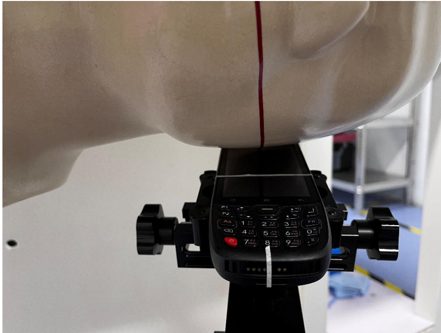
Left Head Tilt (15° ) (0mm)
