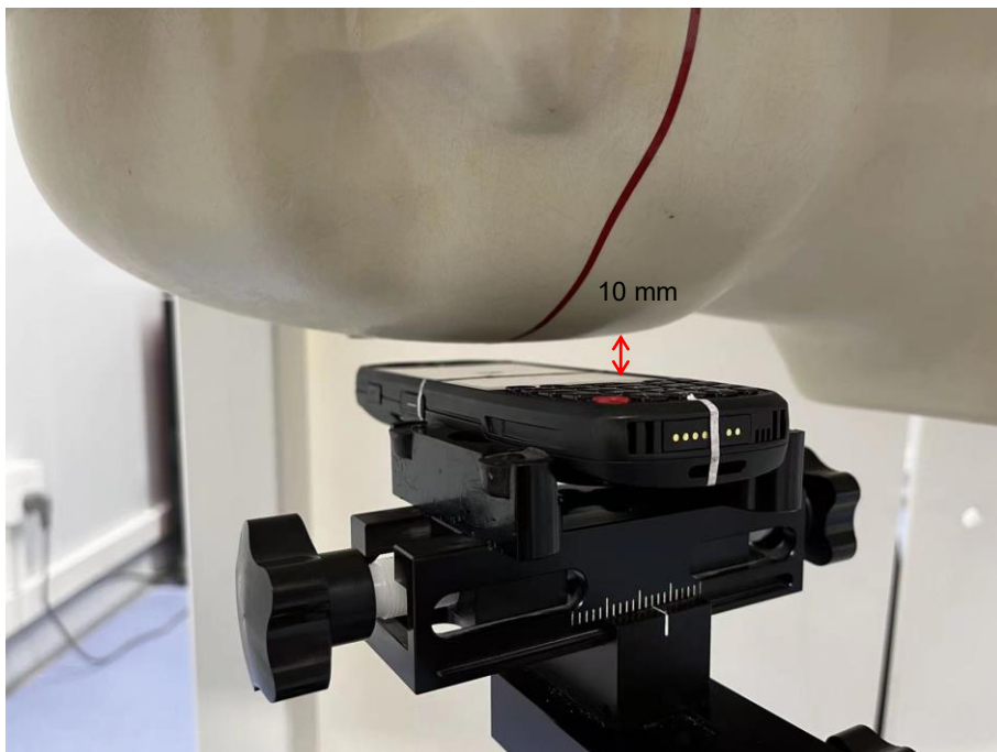
Right Head Cheek (10mm)
