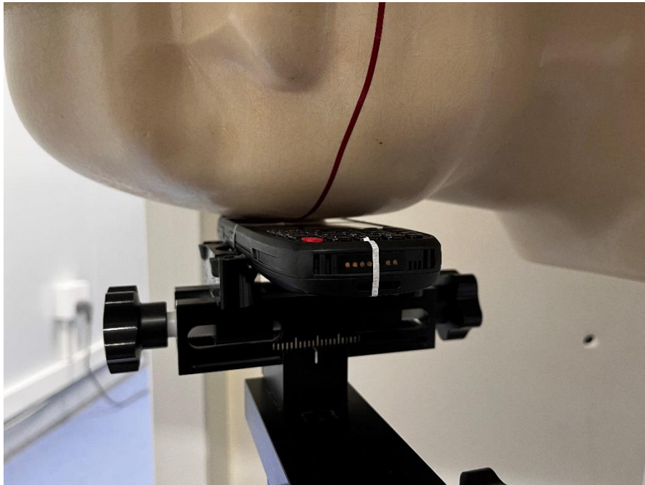
Right Head Cheek (0mm)
