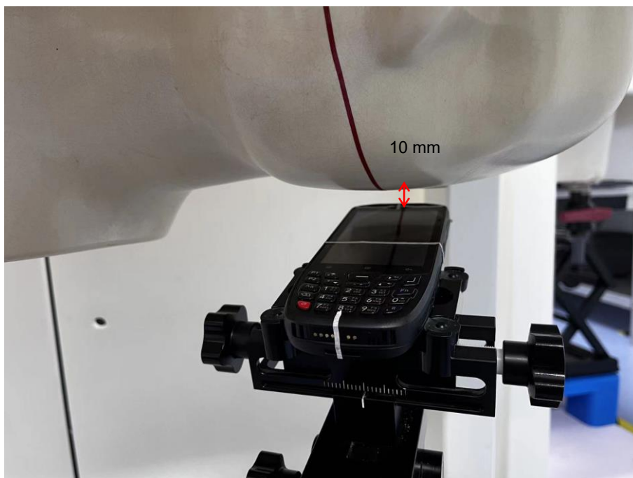
Left Head Tilt (15° ) (10mm)
