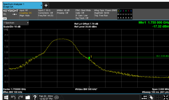
Band4-5MHz-QPSK-20375-25RB#0
